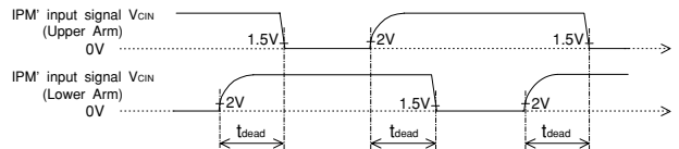
Fig. 7 Dead time measurement point example
