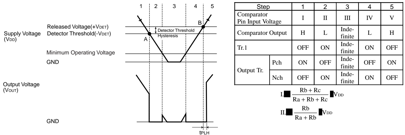
Figure 2. Operation Diagram
