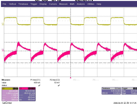
SFS5-12 69mV
