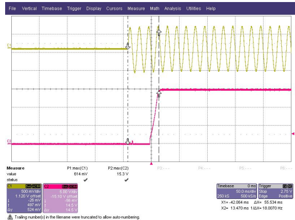
SFS5-15 55.5ms
