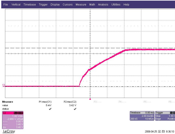
SFS5-3R3 0V
