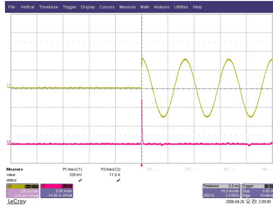
SFS5-5 11.9A
