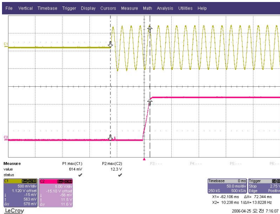
SFS5-12 72.3ms
