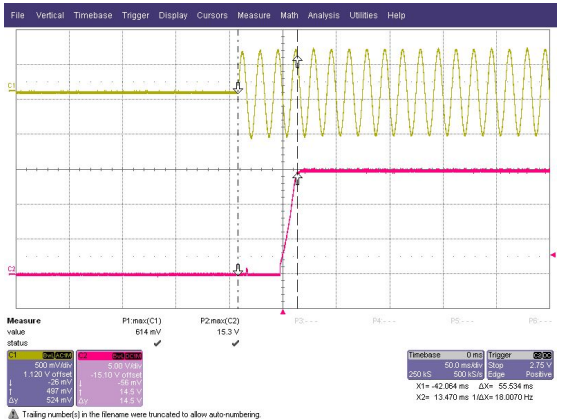
SFS5-24 32.9ms
