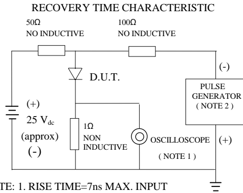
FIG. 1-TEST CIRCUIT DIAGRAM AND REVERSE
