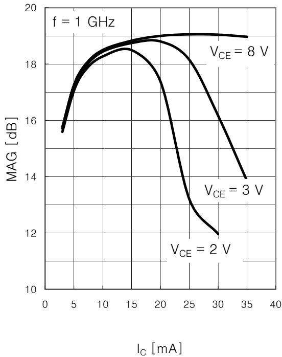
Maximum Available Gain, MAG vs. I C
