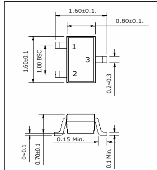
SOT 523 Unit in mm
