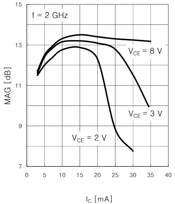
Maximum Available Gain, MAG vs. I C
