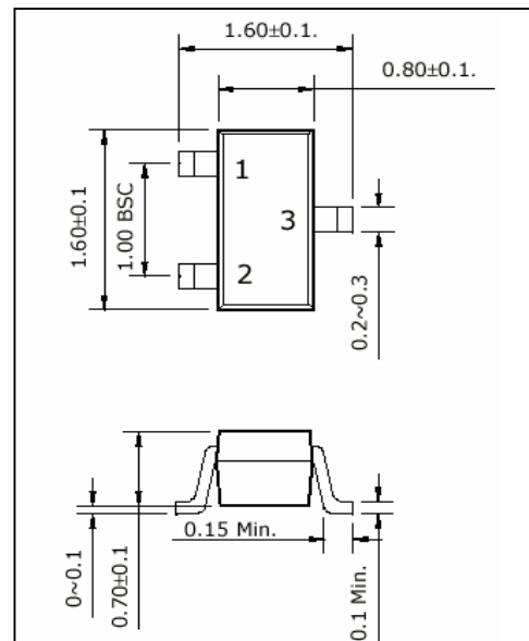
SOT-523 Unit in mm
