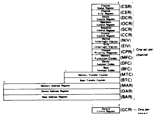
Figure 10 Internal Registers
