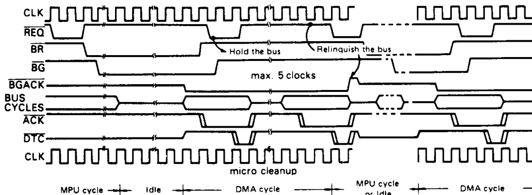
Figure 17 Cycle Steal Mode Request Timing
