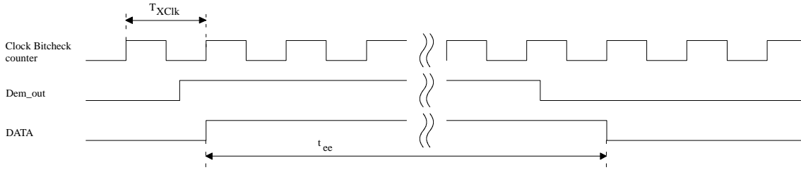
Figure 16. Synchronization of the demodulator output
