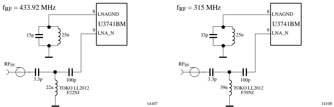
Figure 6. Input matching network without SAW filter
