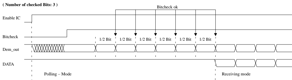
Figure 11. Timing diagram for complete successful bitcheck
