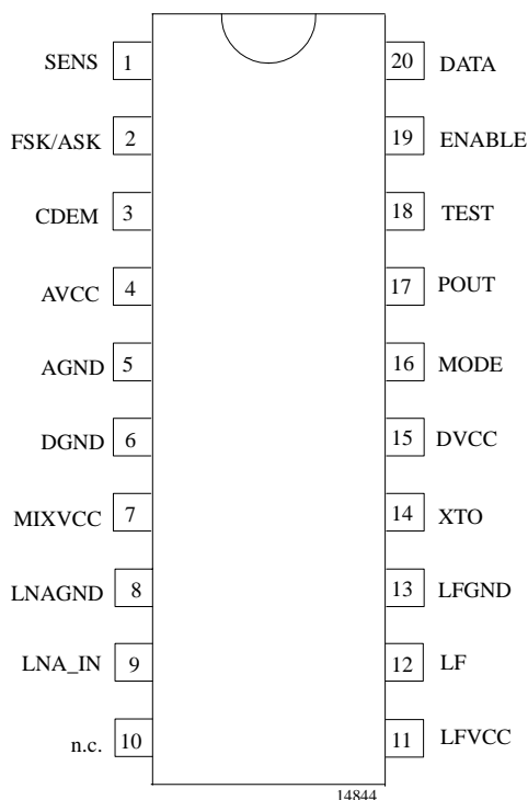
Figure 2. Pinning SO20
