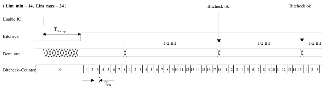
Figure 13. Timing diagram during bitcheck
