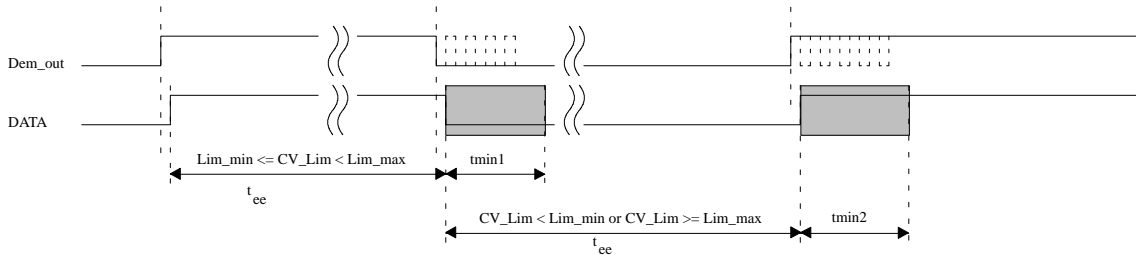
Figure 17. Debouncing of the demodulator output
