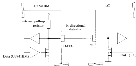
Figure 23. One wire connection to a µC
