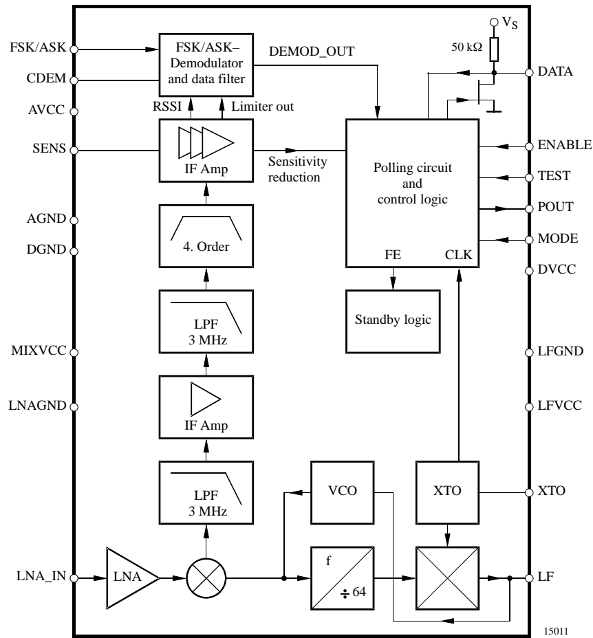
Figure 3. Block diagram
