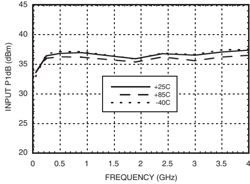
Input P1dB vs. Temperature, Vctl = 0/+3V
