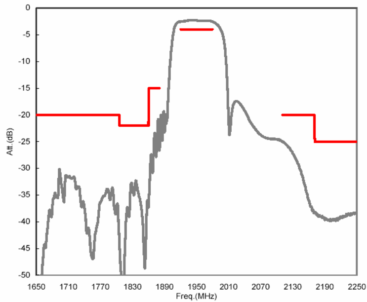
Frequency Response
