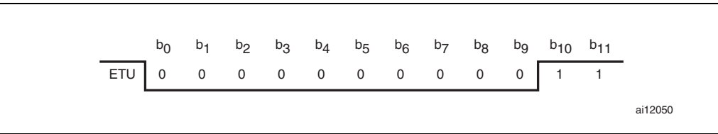
Figure 21. Request start of frame
