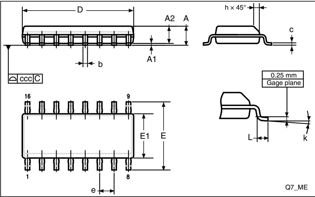
Figure 36. SO16 narrow - 16 lead plastic small outline, 150 mils body width, Package outline
