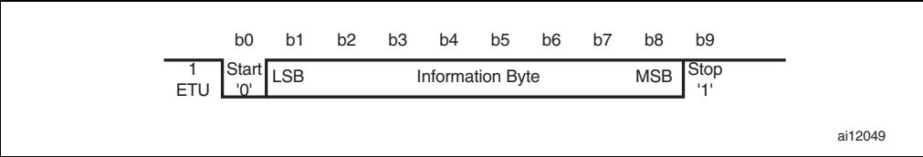
Figure 20. CR14 request frame character format
