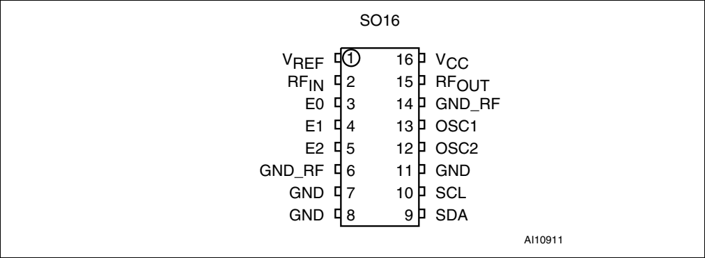
Figure 3. SO pin connections
