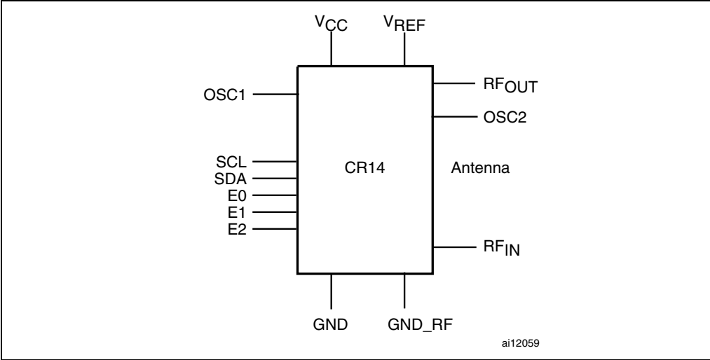
Figure 1. Logic diagram
