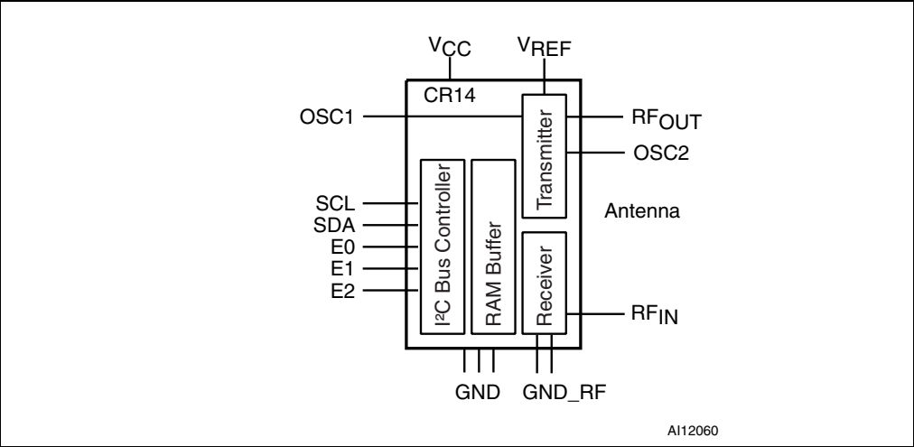
Figure 2. Logic block diagram
