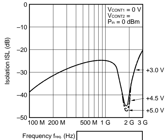
IN-OUT2 ISOLATION vs. FREQUENCY
