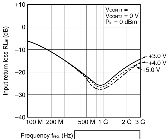
IN-OUT2 RETURN LOSS vs. FREQUENCY
