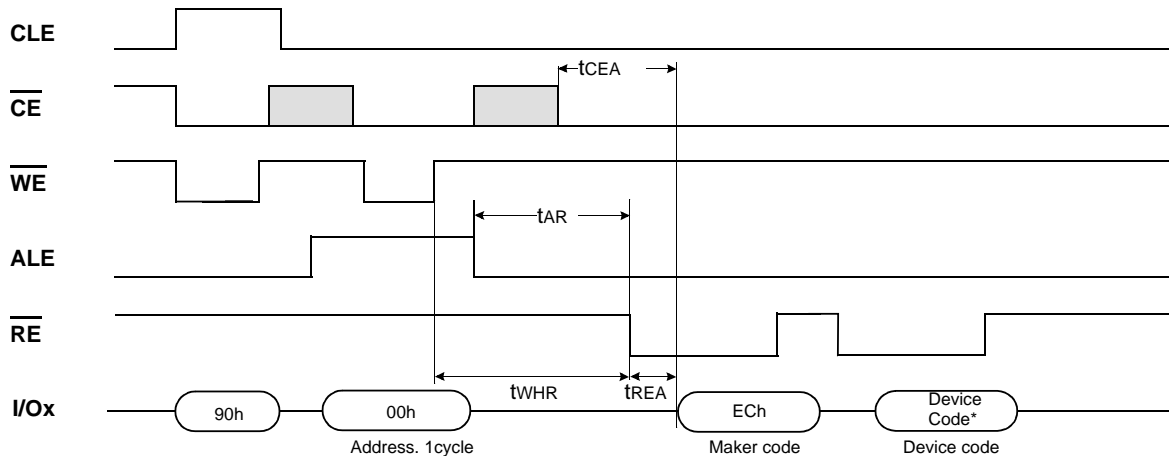
Figure 13. Read ID Operation
