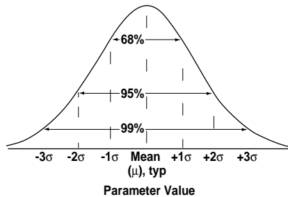
Figure 30. Normal Distribution.
