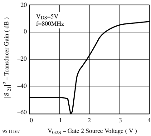
95 11167 Figure 7. Transducer Gain vs. Gate 2 Source Voltage
