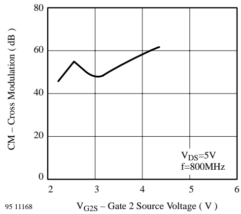
95 11168 Figure 8. Cross Modulation vs. Gate 2 Source Voltage
