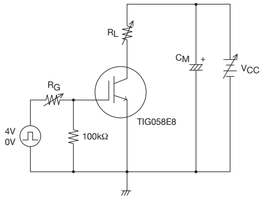
Fig.1 Large Current R Load Switching Circuit
