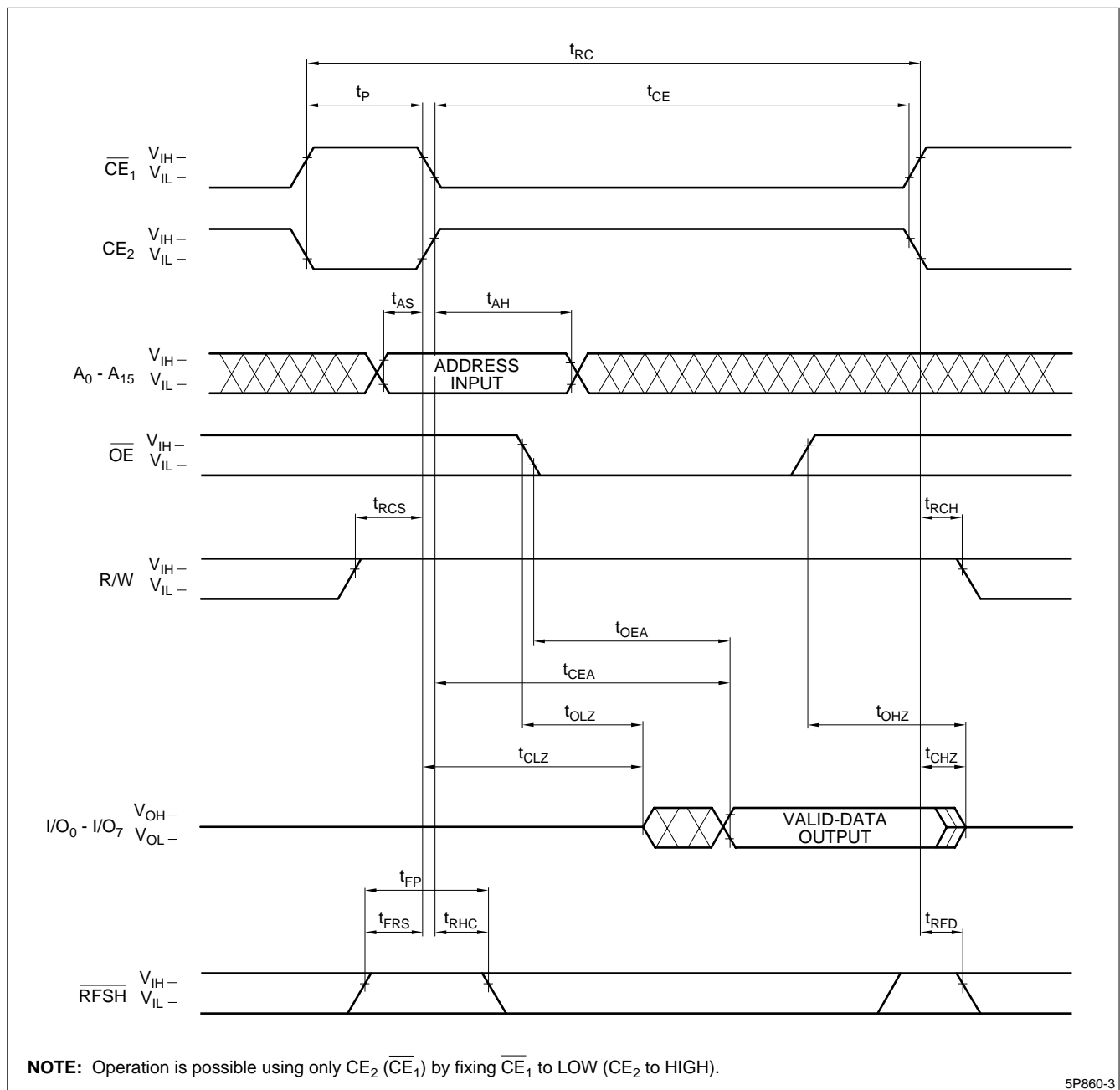
Figure 4. Read Cycle
