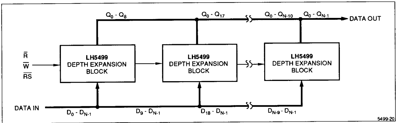
Figure 20. Compound FIFO
