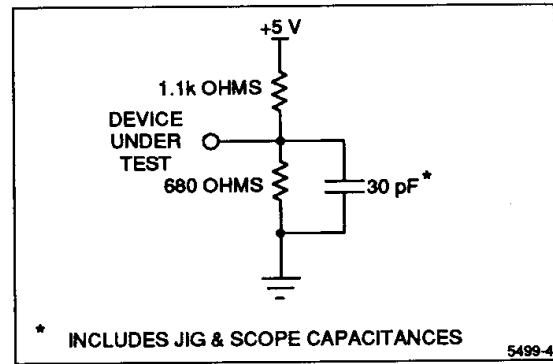
Figure 4. Output Load Caption
