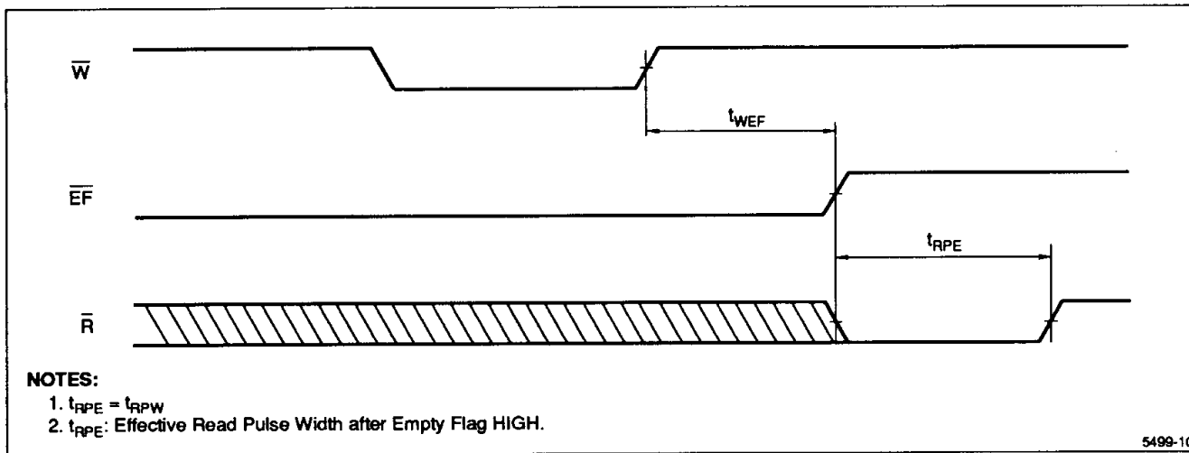
Figure 11. Empty Flag Timing
