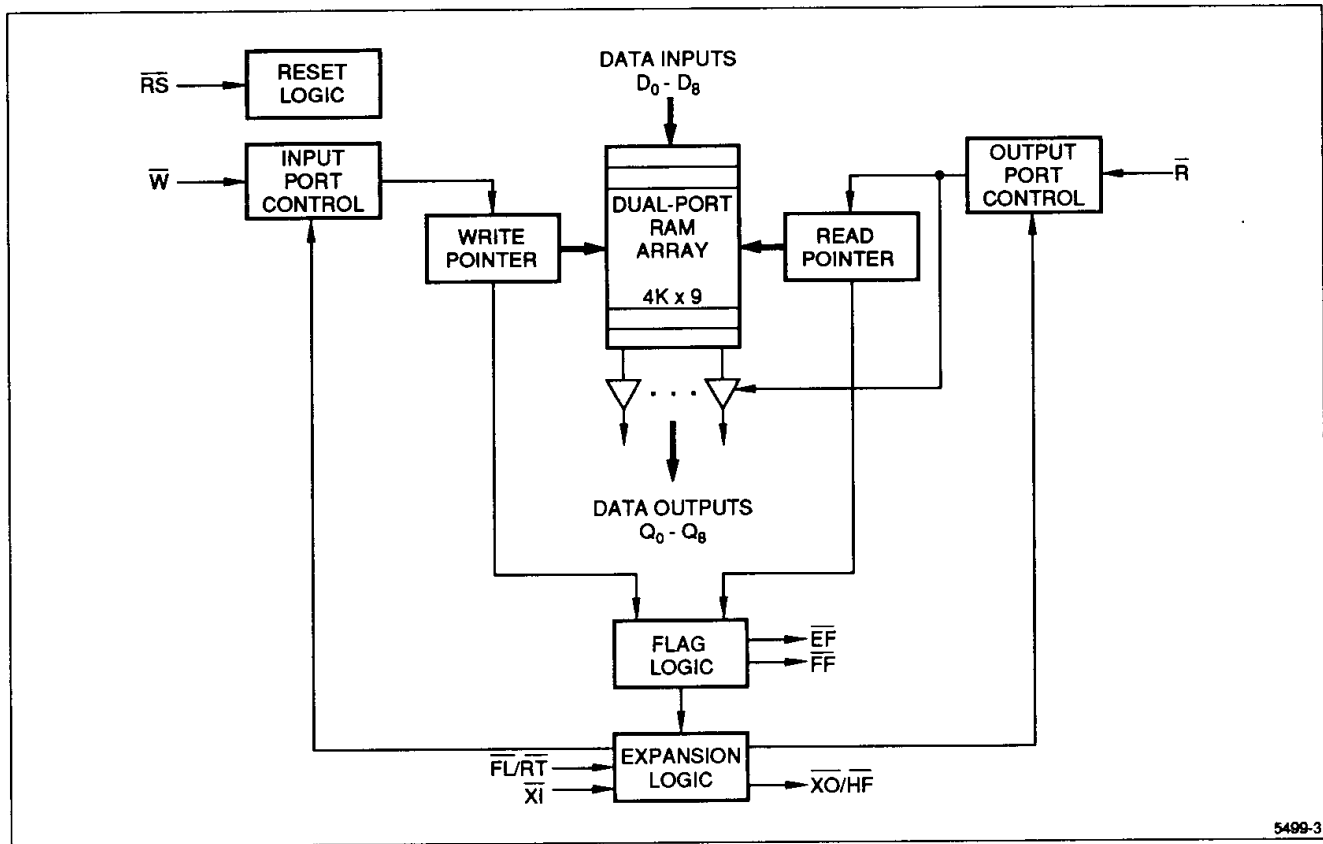
Figure 3. LH5499 Block Diagram
