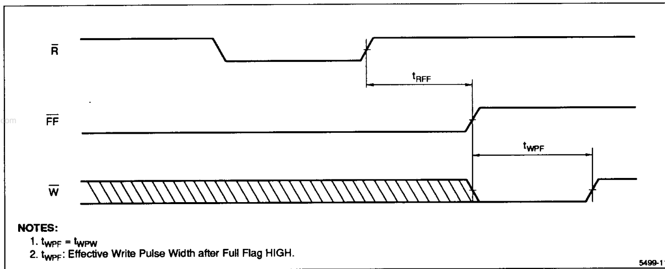
Figure 12. Full Flag Timing
