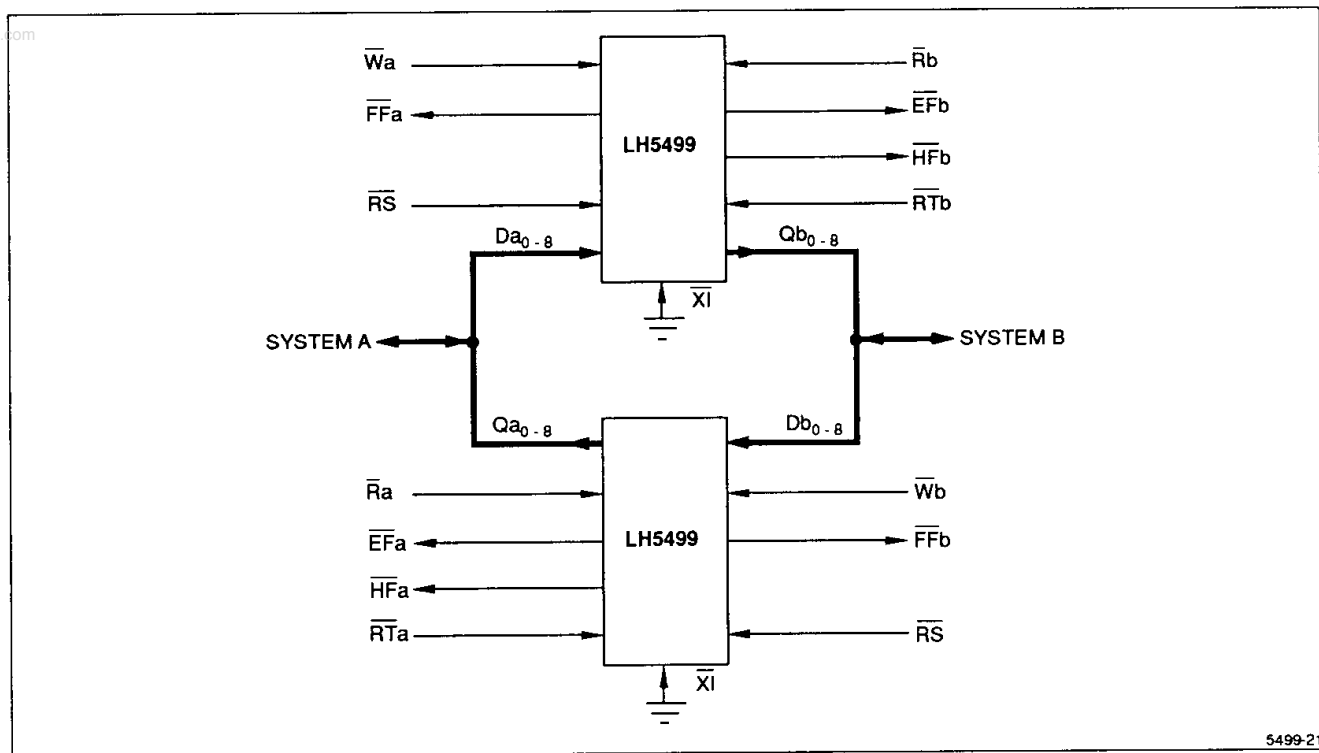
Figure 21. Bidirectional FIFO
