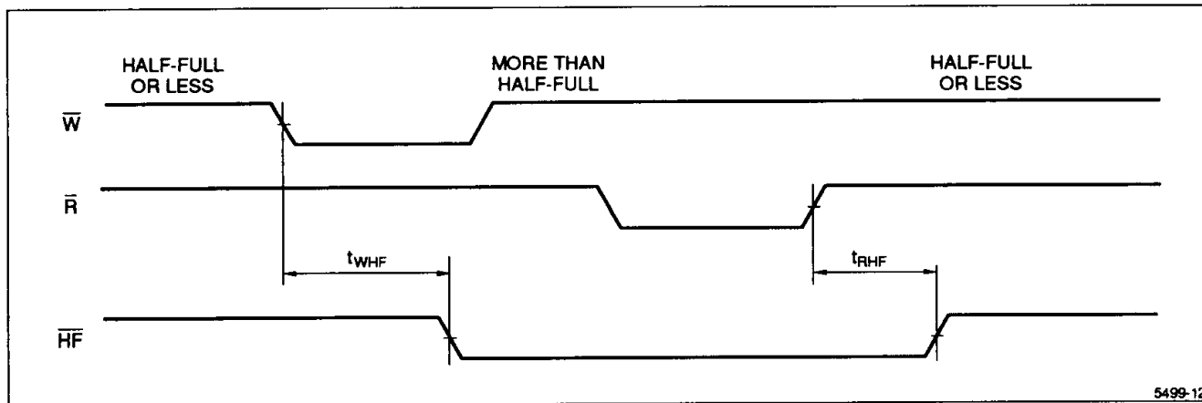
Figure 13. Half-Full Flag Timing
