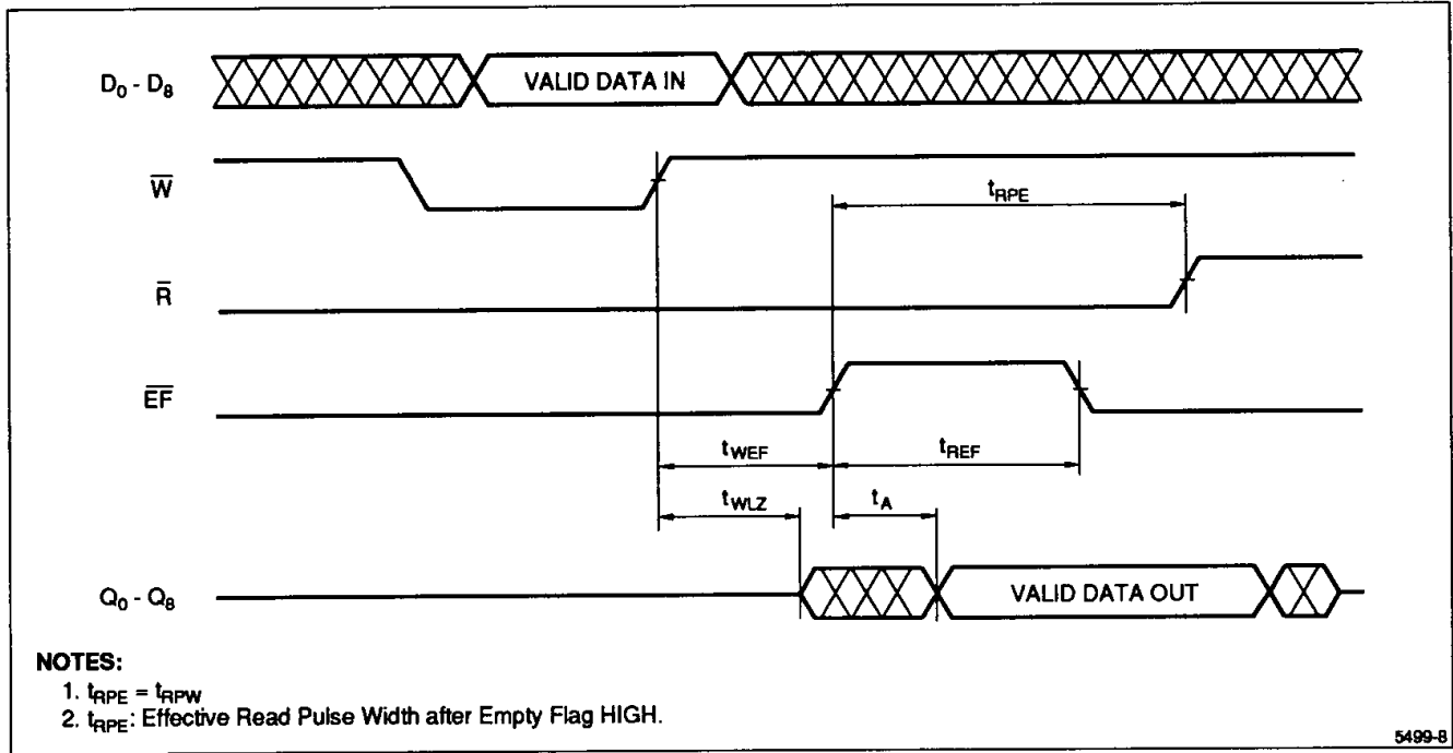
Figure 9. Read Data Flow-Through
