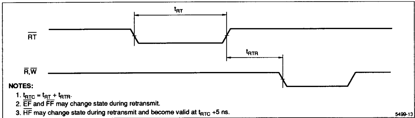
Figure 14. Retransmit Timing
