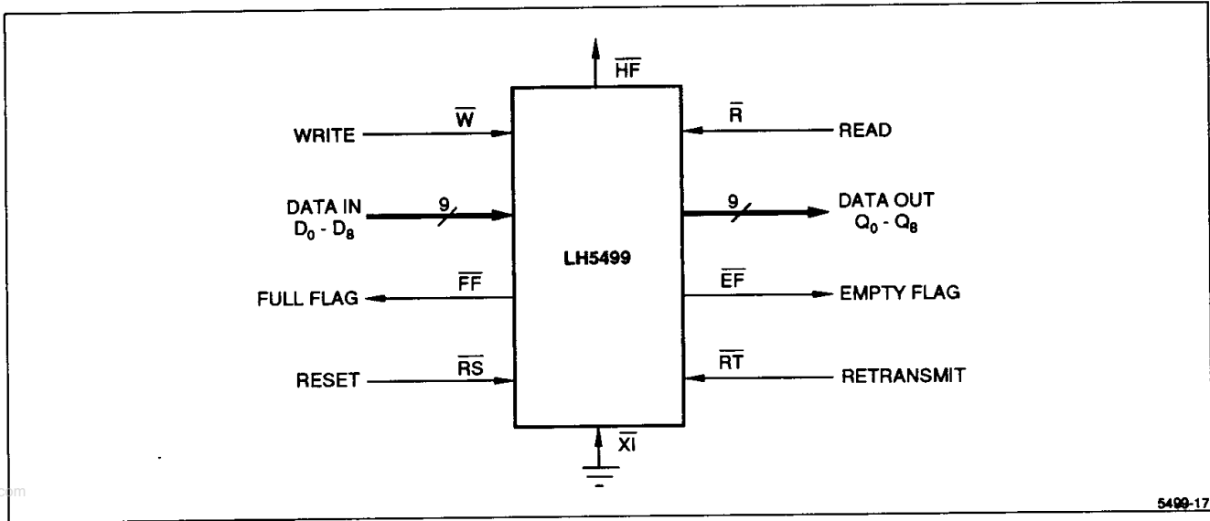
Figure 17. Single FIFO (4K × 9)
