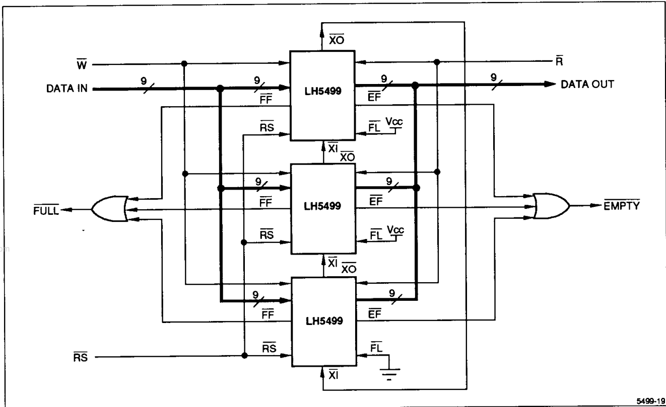
Figure 19. FIFO Depth Expansion (12288 × 9)
