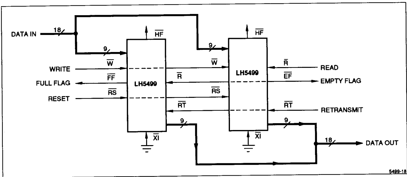
Figure 18. FIFO Width Expansion (4K × 18)
