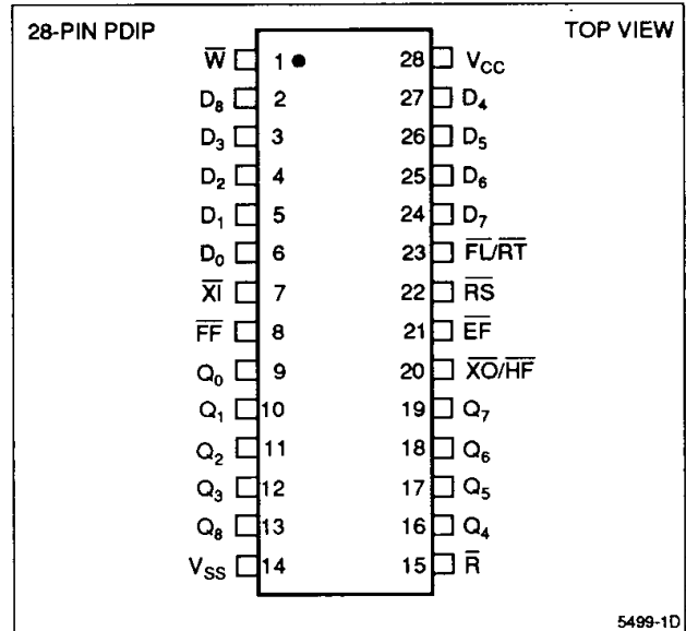
Figure 1. Pin Connections for PDIP Package
