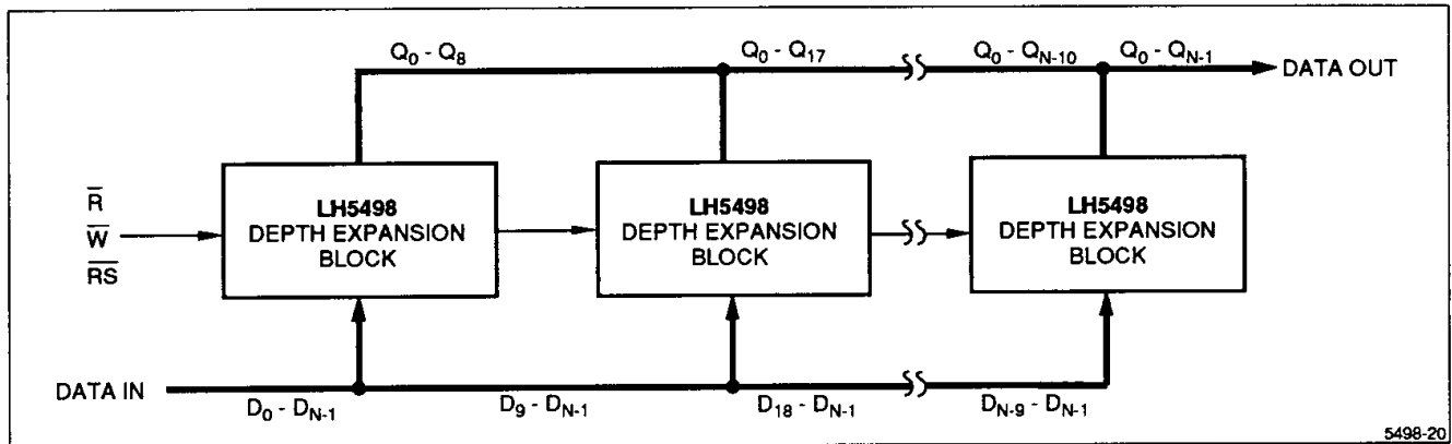
Figure 20. Compound FIFO
