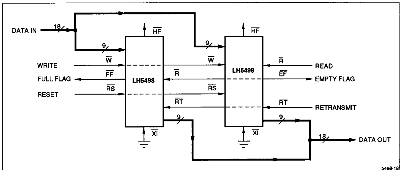
Figure 18. FIFO Width Expansion (2K × 18)
