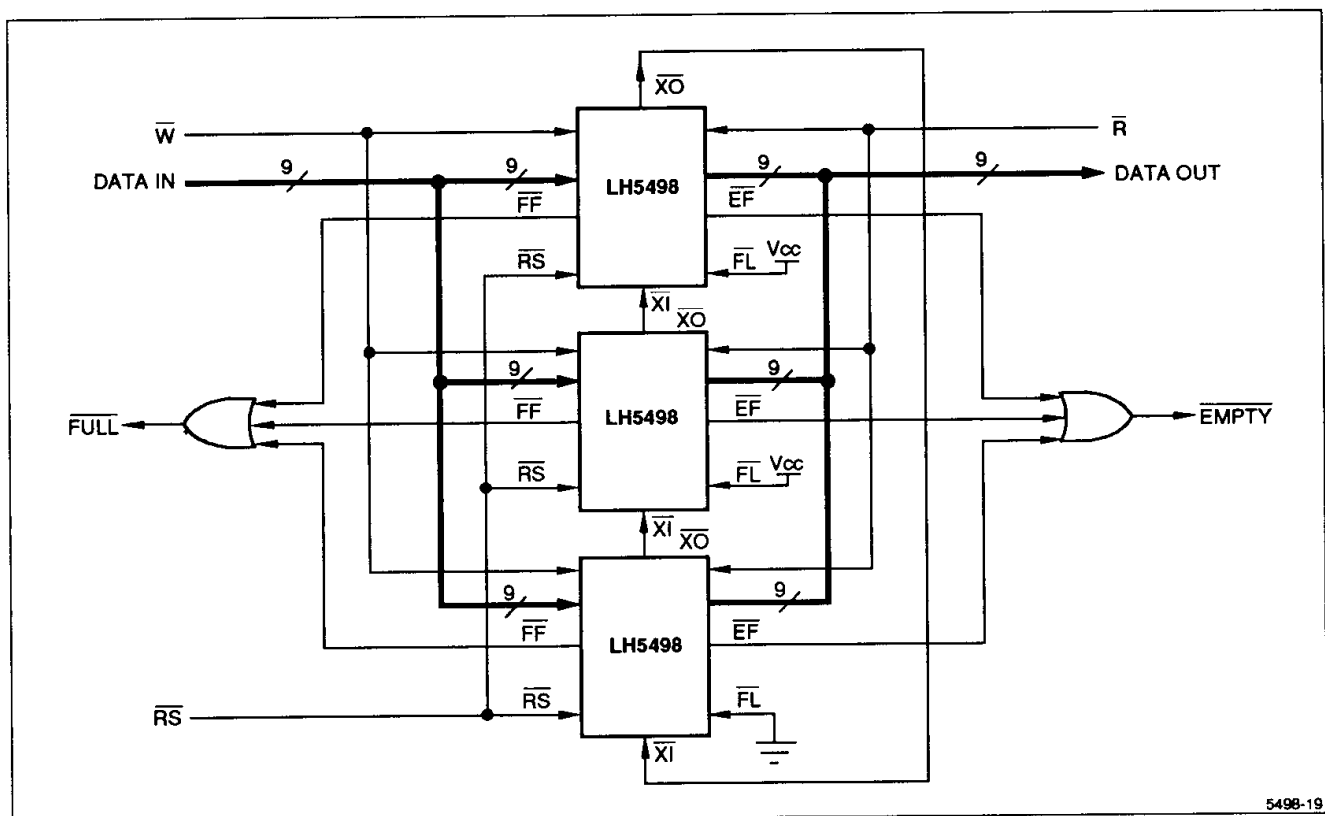
Figure 19. FIFO Depth Expansion (6144 × 9)
