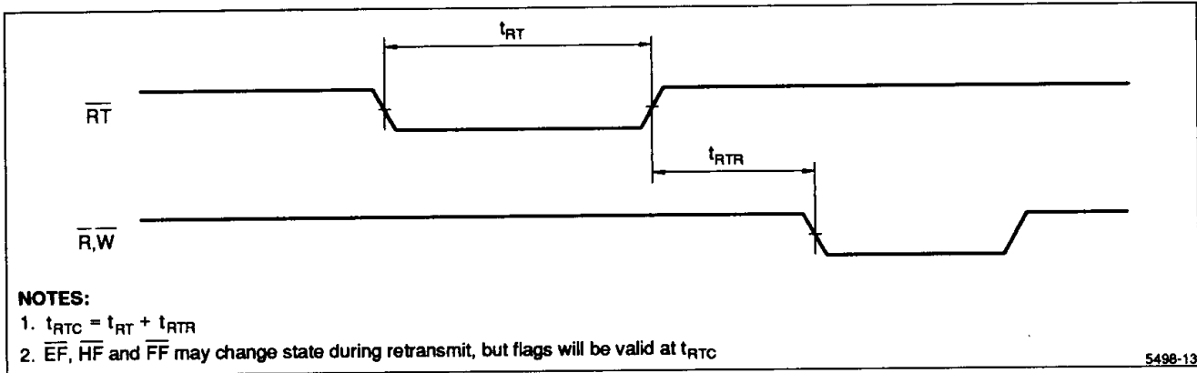
Figure 14. Retransmit Timing
