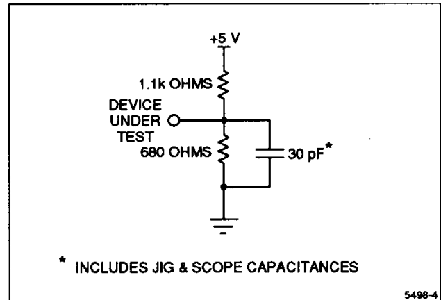
Figure 4. Output Load Circuit
