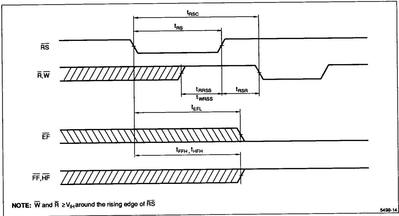
Figure 5. Reset Timing
