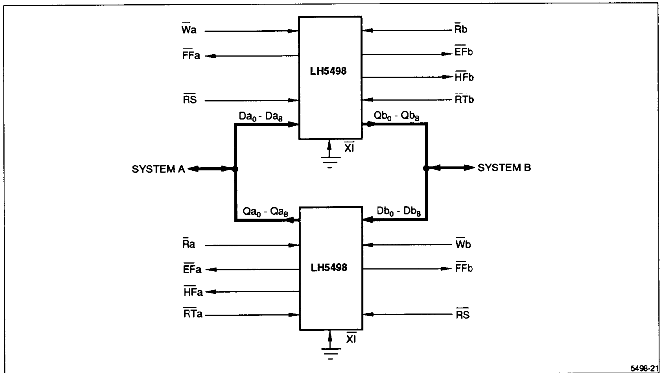
Figure 21. Bidirectional FIFO
