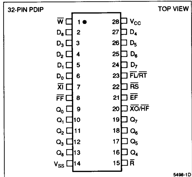
Figure 1. Pin Connections for DIP Package
