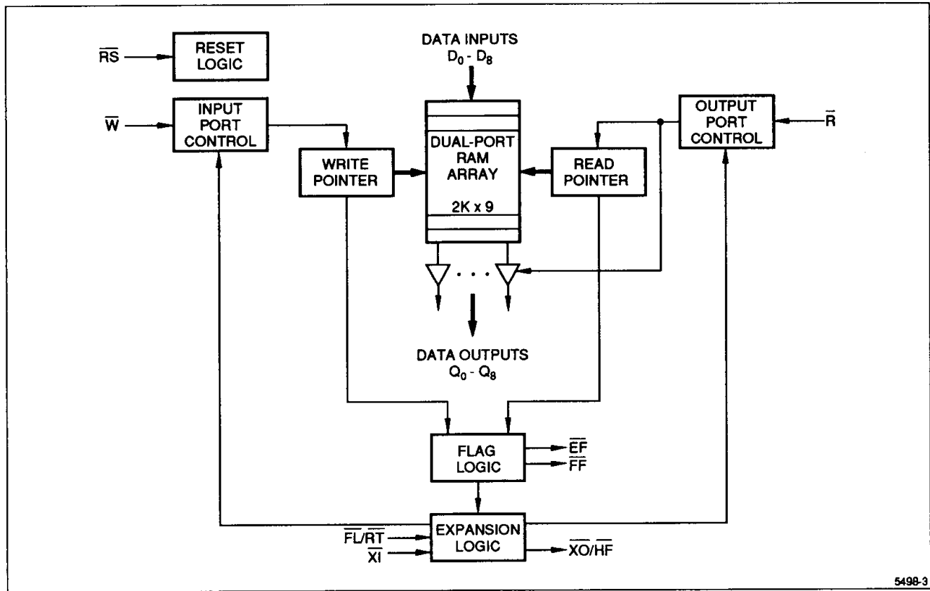
Figure 3. LH5498 Block Diagram
