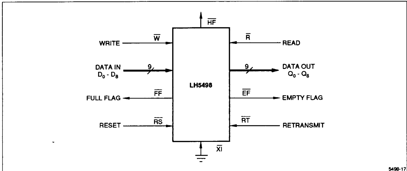
Figure 17. Single FIFO (2K × 9)
