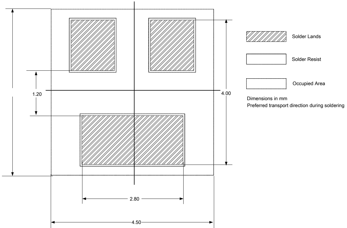
Figure 6. Waving Soldering Footprint SOT-23
