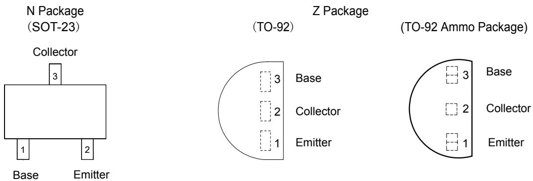
Figure 2. Pin Configurations of APT17 (Top View)
