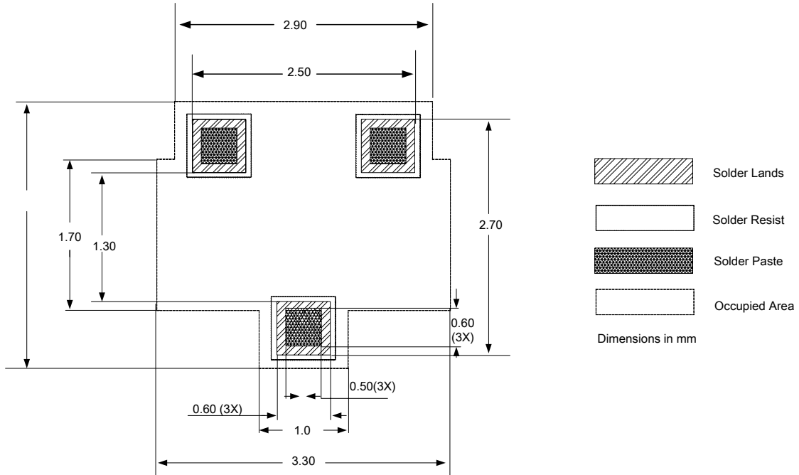
Figure 5. Reflow Soldering Footprint SOT-23
