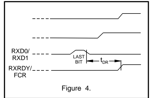
RECEIVER OPERATION
