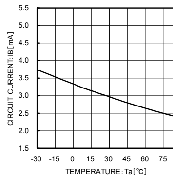
Fig.12 Circuit Current vs Temperature
