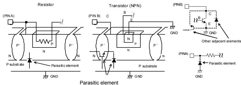
Fig. 33 Example of Simple Bipolar IC Architecture
