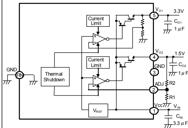
Fig.25 BA3259HFP Block Diagram
