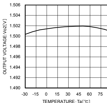
Fig.11 Output Voltage vs Temperature (Variable output: 1.5 V)
