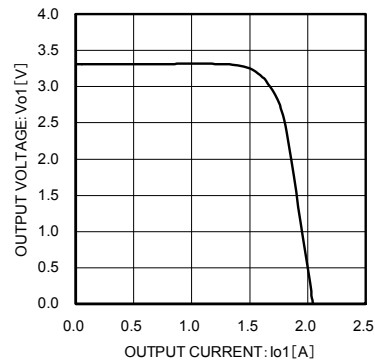
Fig.6 Load Stability (3.3 V output)
