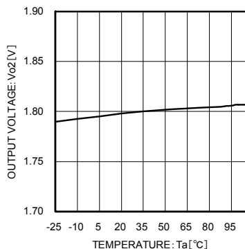
Fig. 23 Output Voltage vs Temperature (Variable output: 1.8 V)
