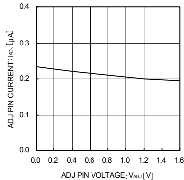
Fig. 15 ADJ Pin Source Current
