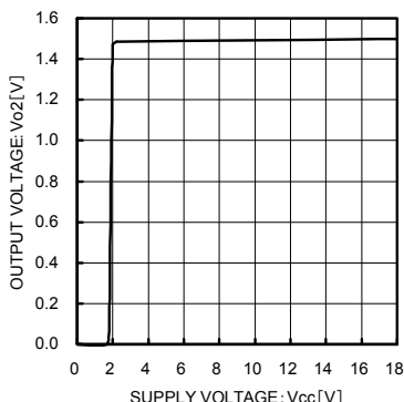
Fig. 17 Input Stability (Variable output: 1.8 V)
