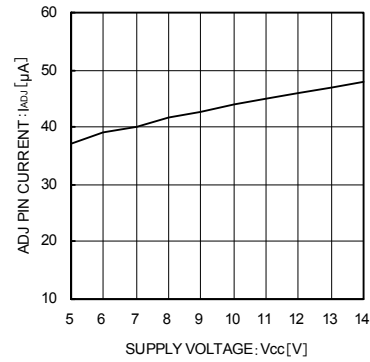
Fig.3 ADJ Pin Outflow Current
