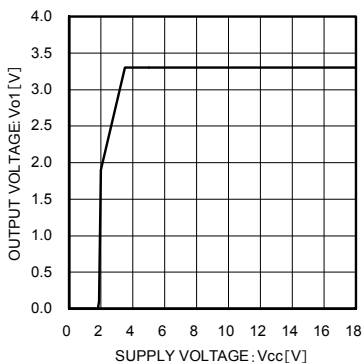
Fig. 16 Input Stability (3.3 V output I O1 =600 mA)
