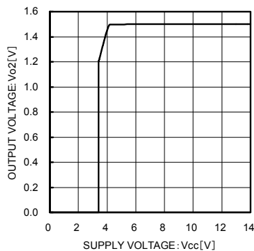
Fig.5 Input Stability (Variable output with no load)
