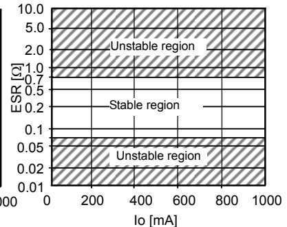
Fig.29 BA30E00WHFP ESR
