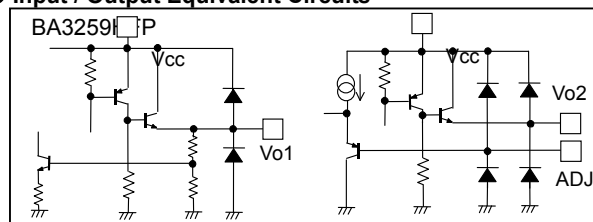
Fig.30 BA3259HFP I/O Equivalent Circuits
