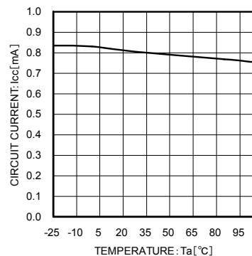
Fig. 24 Circuit Current vs Temperature (I O =0 mA)
