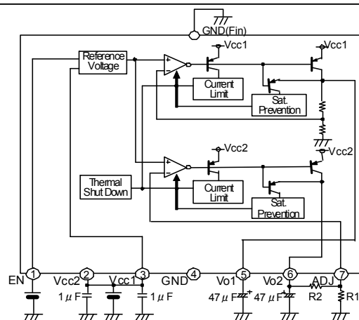
Fig.26 BA30E00WHFP Block Diagram
