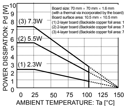
Fig. 27 Ambient Temperature vs. Power Dissipation
