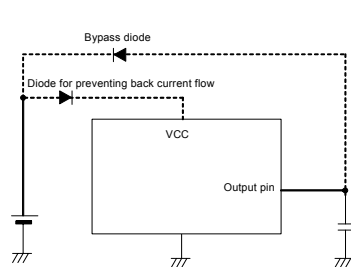
Fig. 32 Bypass diode
