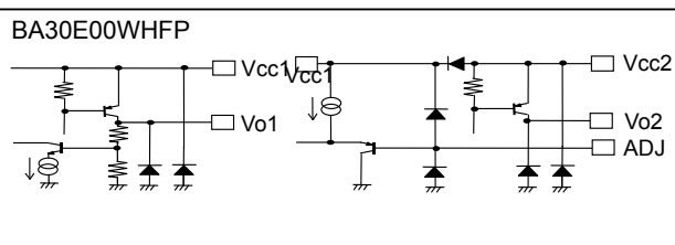
Fig.31 BA30E00WHFP I/O Equivalent Circuit
