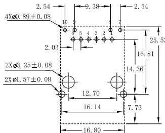
PC Board Layout Component Side Shown
