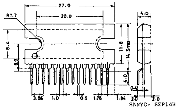
Case Outline 3082-S14HIC (unit: mm)
