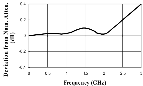
Attenuation Accuracy, 8 dB
