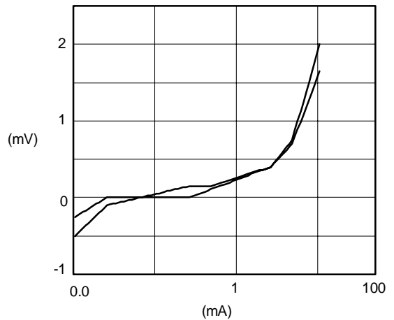
Forward Characteristic
