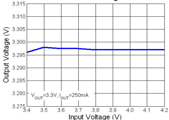
CH1 Buck Line Regulation
