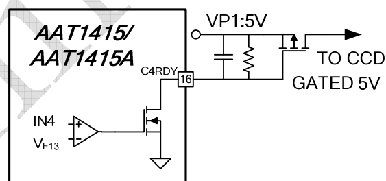
Figure 4. C4RDY Application Circuit
