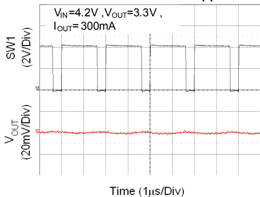
CH1 Buck SW1 and Ripple
