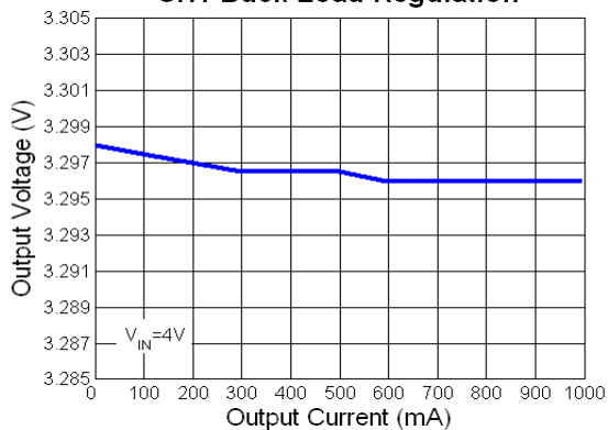
CH1 Buck Load Regulation
