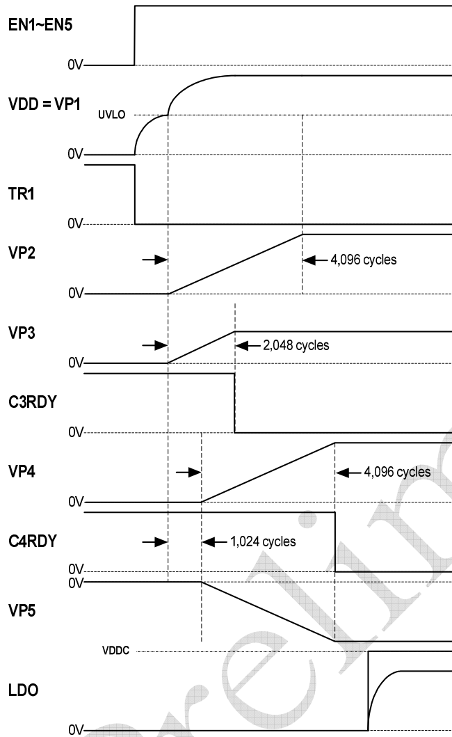
Figure 7. Timing Chart of Soft-Start
