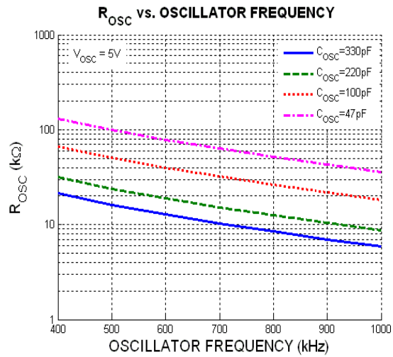
Figure 8. Oscillator Frequency
