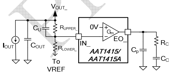
Figure 9b. Feedback Network (For Inverting)
