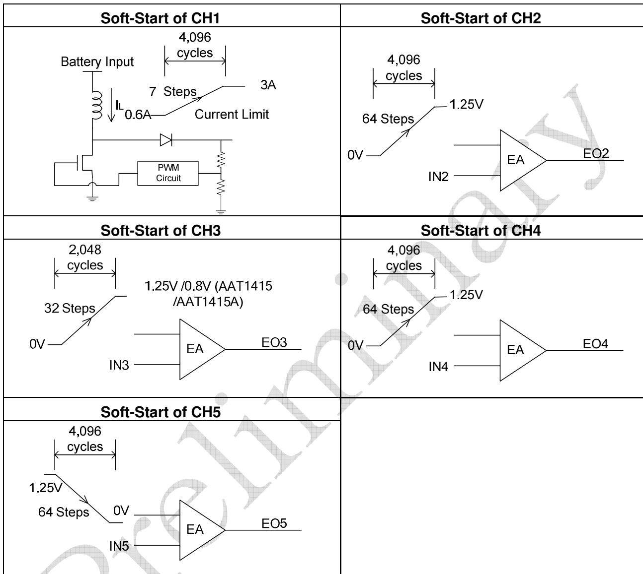
Figure 6. Soft-Start Mechanism
