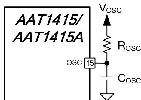
Figure 5. Oscillator Circuit
