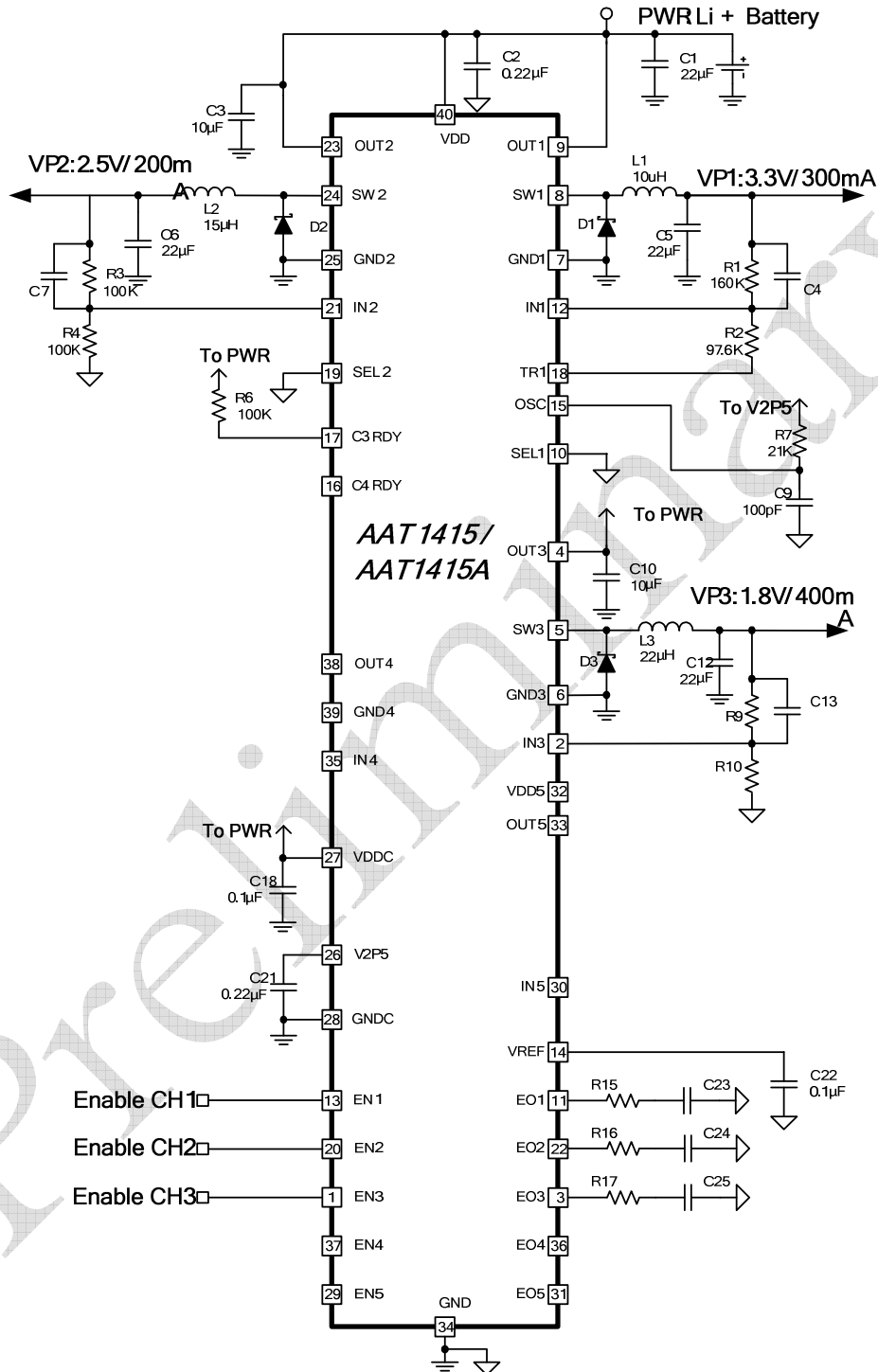
Figure 3. Typical 1-Cell Li+ Powered System (For CMOS)
