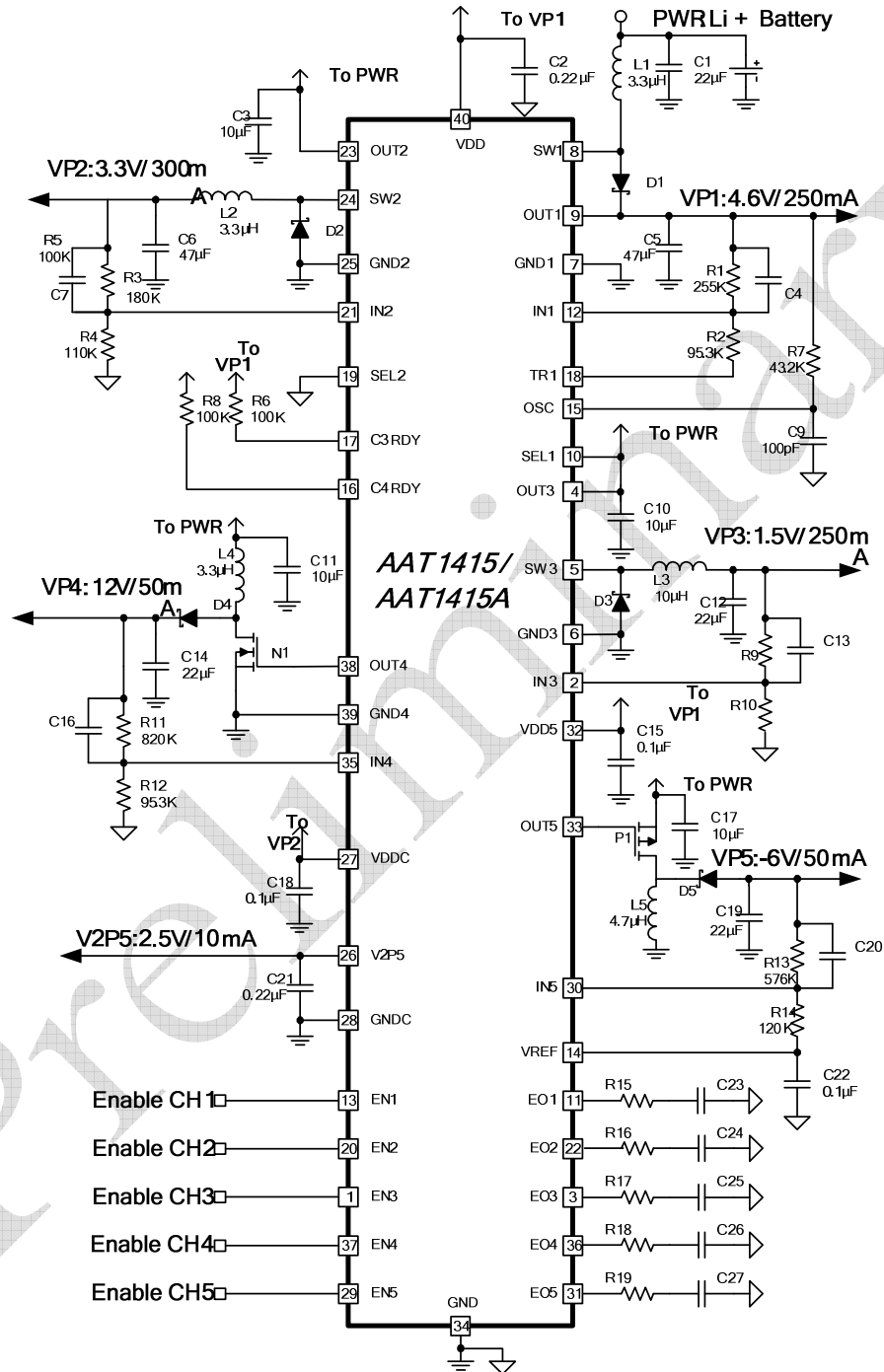
Figure 2. Typical 1-Cell Li+ Powered System (For CCD)
