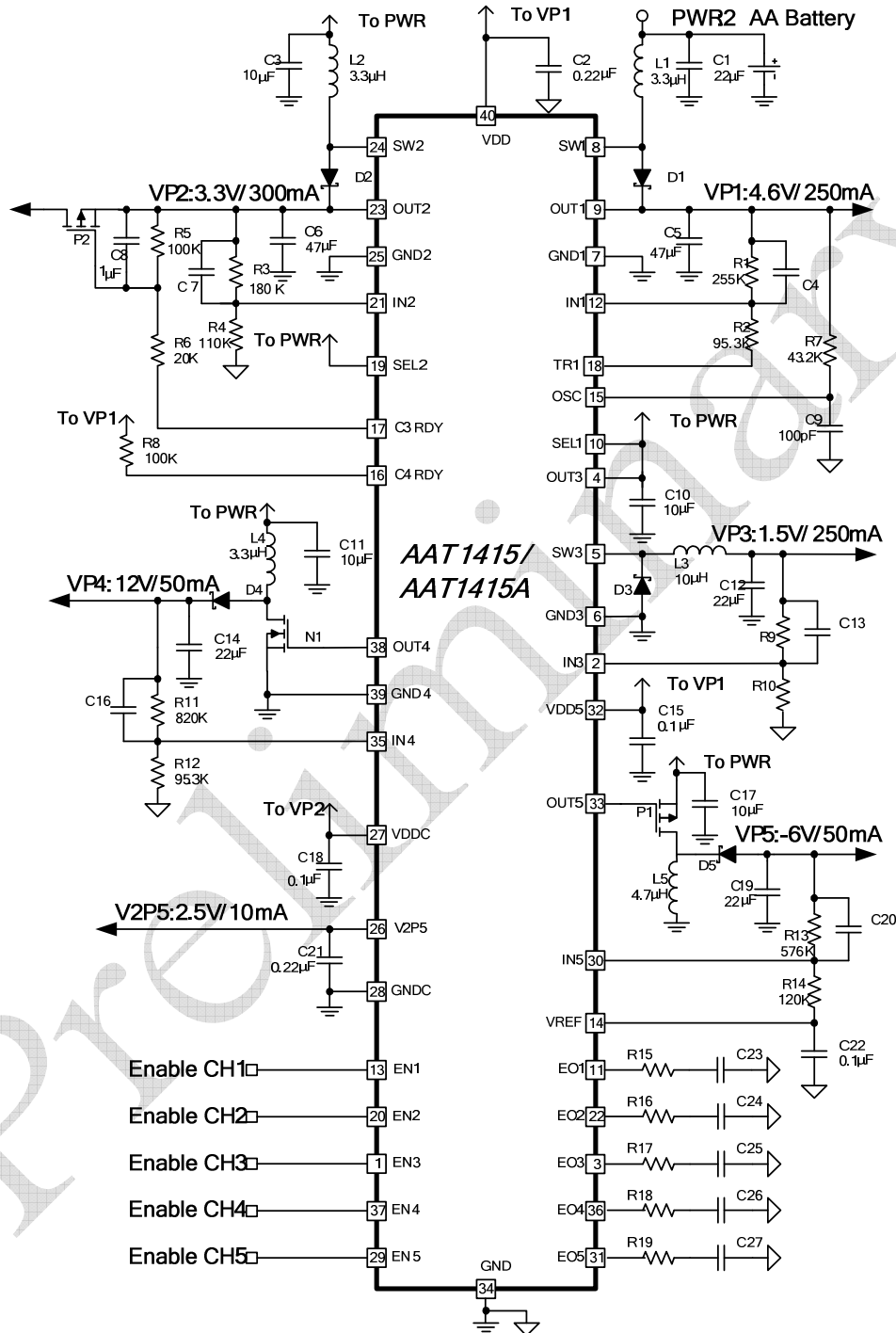
Figure 1. Typical 2-Cell AA-Powered System
