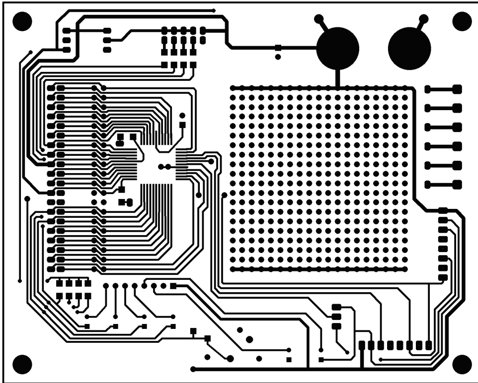
Figure 5. Top-side Foil
