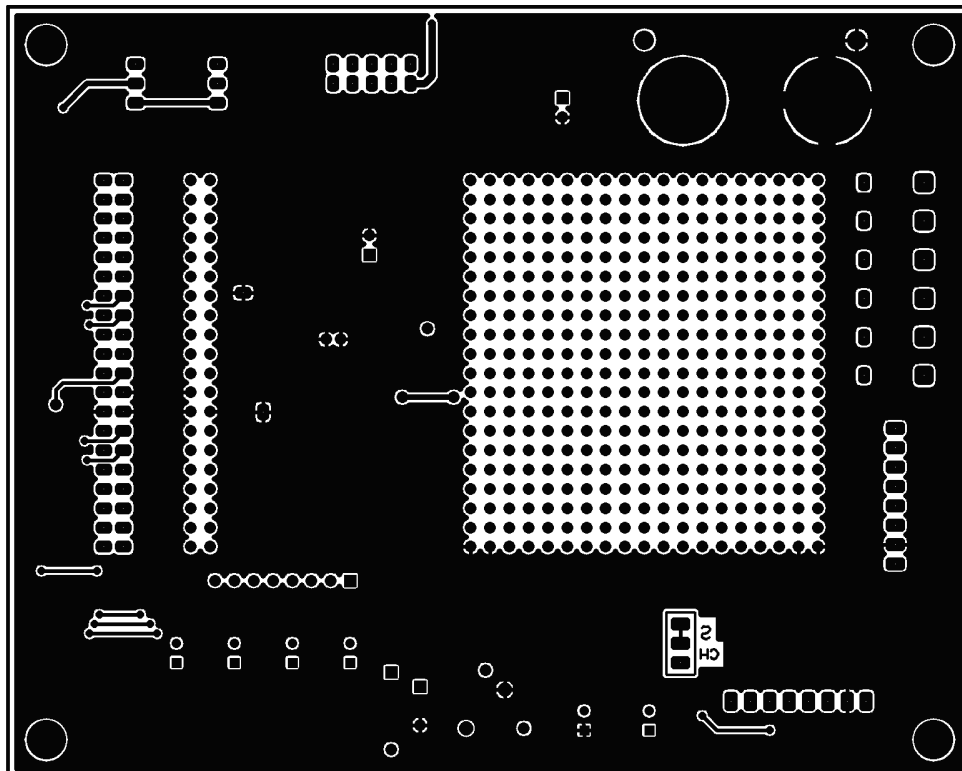
Figure 6. Bottom-side Foil
