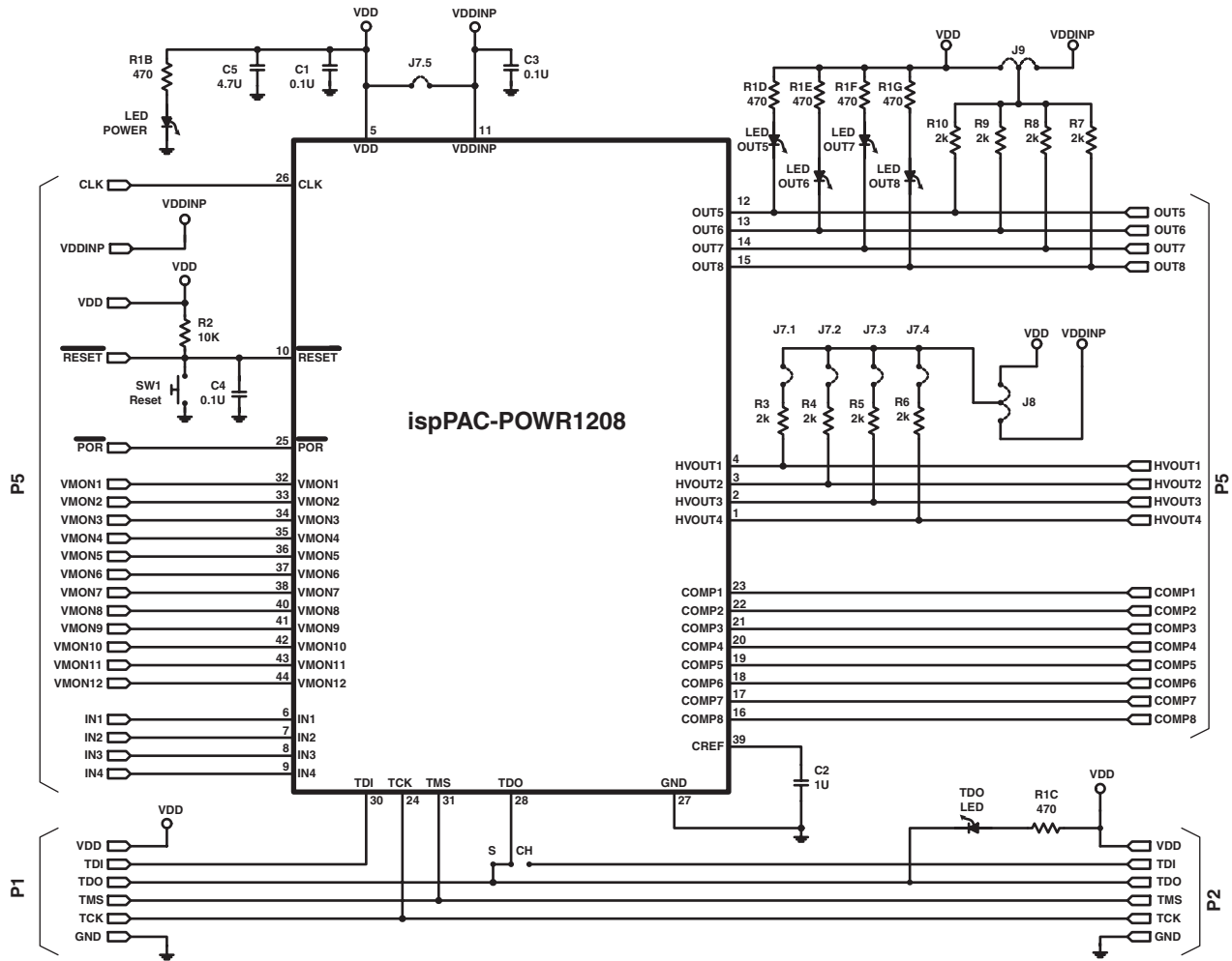
Figure 2. Schematic
