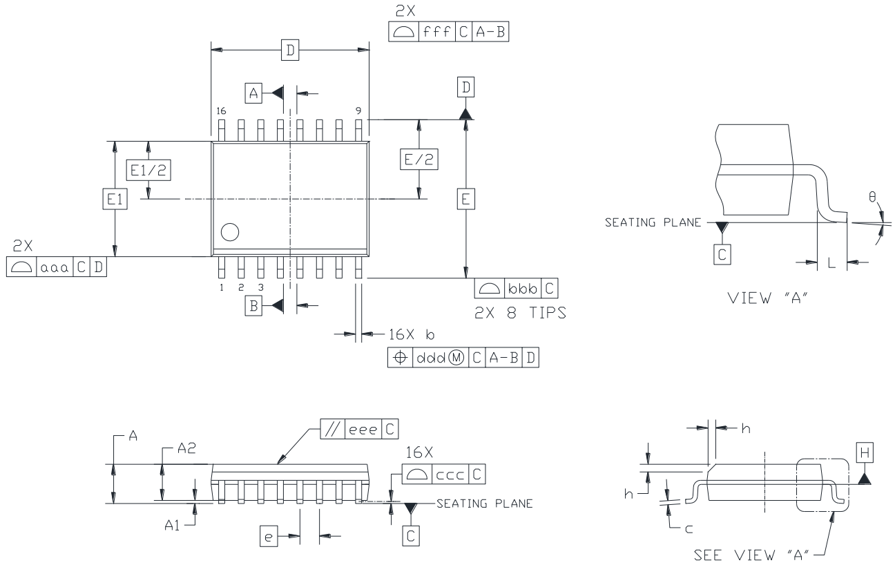
Figure 15. 16-Pin Wide Body SOIC
