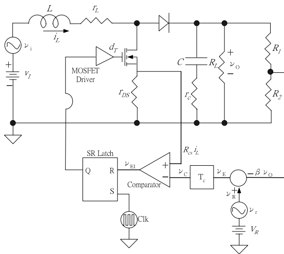
Fig.1. Closed-current loop for boost with PCM
