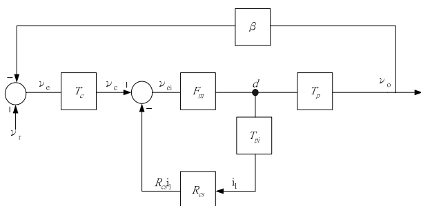
Fig.2. Block diagram of boost converter with PCM
