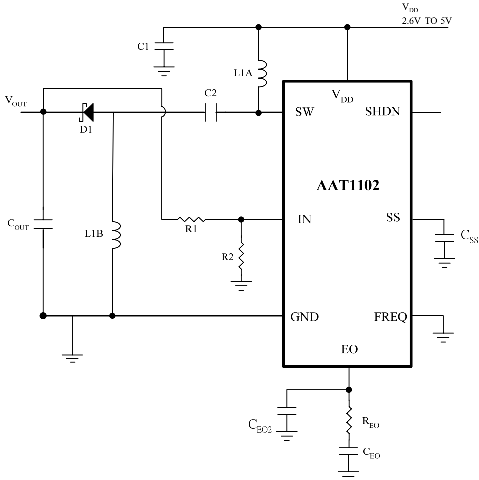
Fig. 3 AAT1102 IN A SEPIC CONFIGURATION
