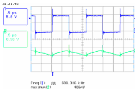
Fig.4. CH1: PWM waveform, CH2, v_{p-p} for V_o
