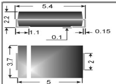
Surface mount diode
