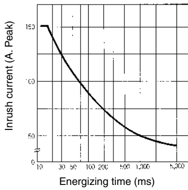
G3PA-210B(L)-VD
