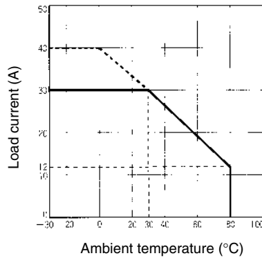
G3PA-430B-VD, G3PA-430B-VD-2
