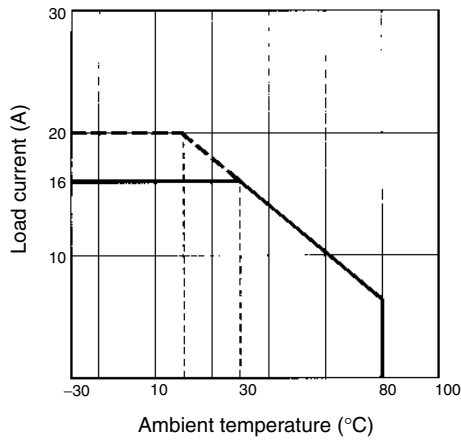
G3PA-450B-VD-2
