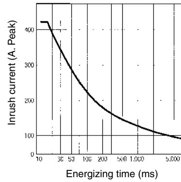
G3PA-240B(L)-VD/260B(L)-VD, G3PA-430B-VD, G3PA-430B-VD-2, G3PA-450B-VD-2
