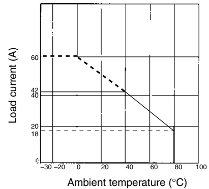
G3PA-260B(L)-VD
