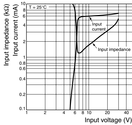
G3PA-4□0-VD, G3PA-4□-VD-2
