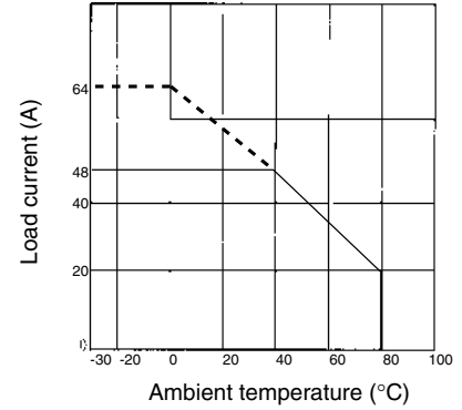
G3PA-260B(L)-VD
