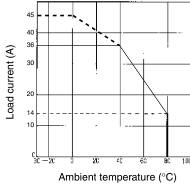
G3PA-430B-VD, G3PA-430B-VD-2
