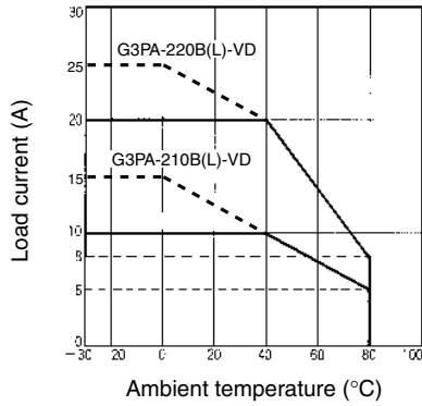
G3PA-210B(L)-VD, G3PA-220B(L)-VD
