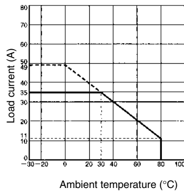
G3PA-450B-VD-2
