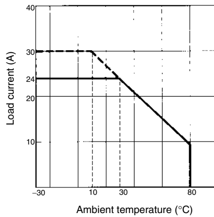
G3PA-430B-VD, G3PA-430B-VD-2
