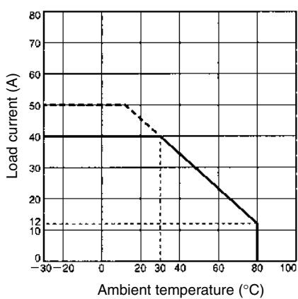
G3PA-450B-VD-2
