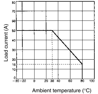
G3PA-450B-VD-2
