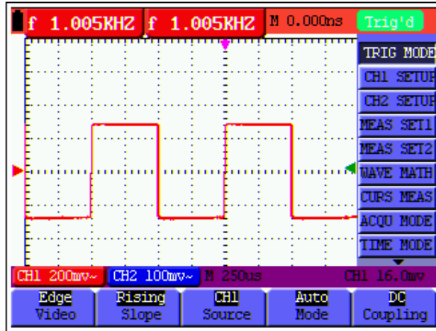
Figure 38: Edge Trigger
