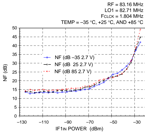
Figure 18. First Mixer and Digital Second IF Section Noise Figure vs. IF1N Power
