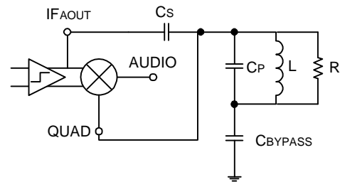
Figure 4. Quadrature Detector
