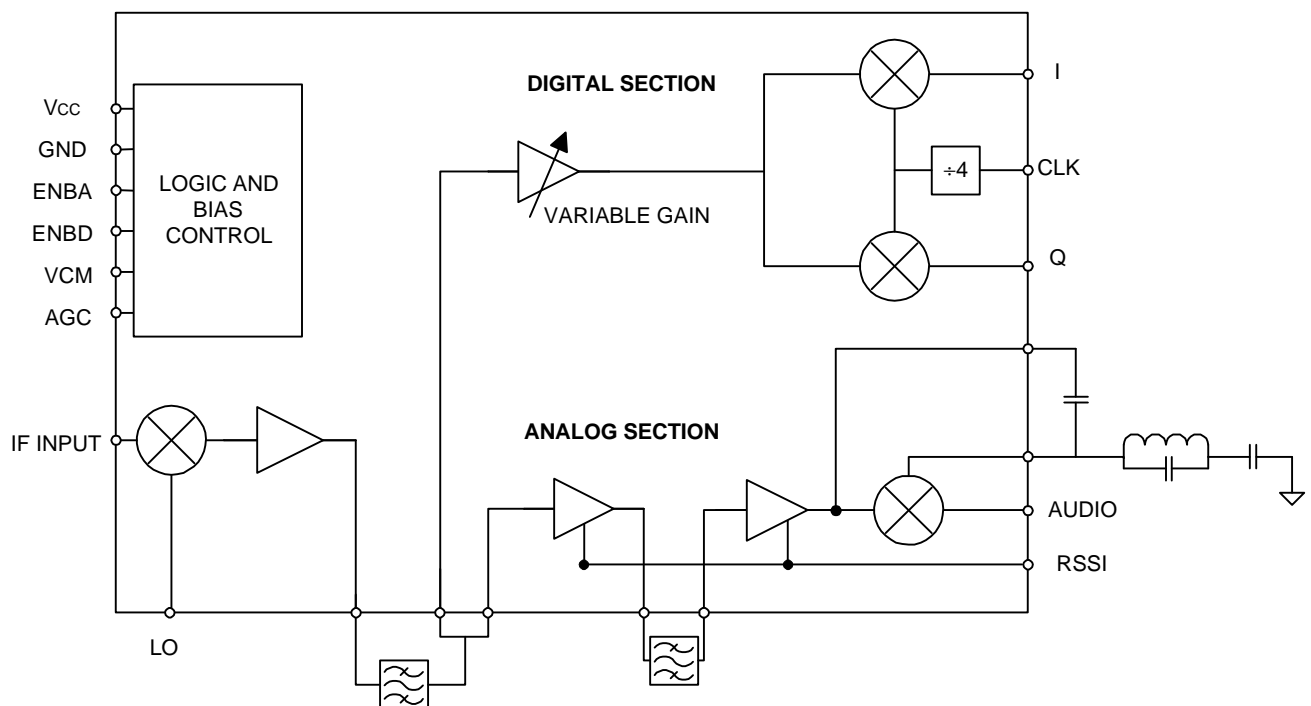
Figure 1. General Block Diagram
