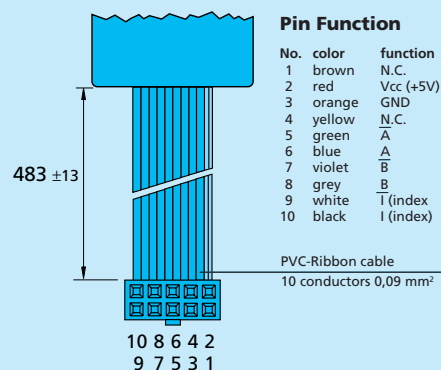
Connector DIN-41651 grid 2,54 mm
