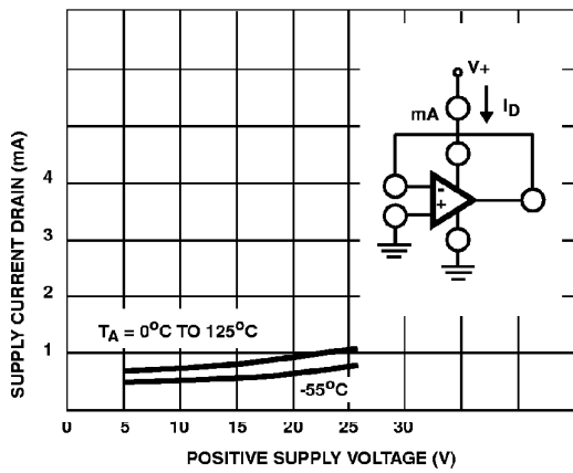
FIGURE 3. SUPPLY CURRENT DRAIN vs SUPPLY VOLTAGE
