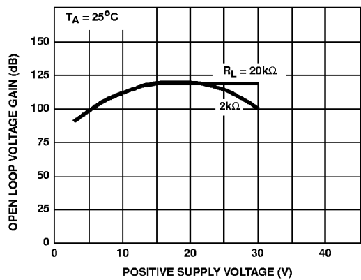
FIGURE 5. VOLTAGE GAIN vs SUPPLY VOLTAGE
