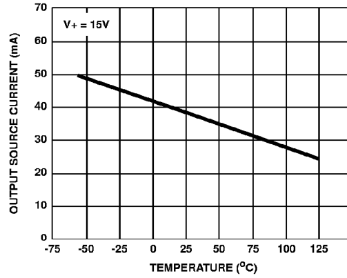
FIGURE 13. OUTPUT CURRENT vs AMBIENT TEMPERATURE
