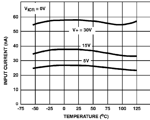
FIGURE 2. INPUT CURRENT vs AMBIENT TEMPERATURE
