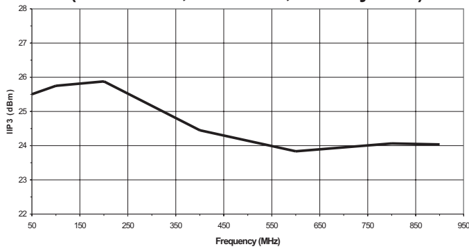
Figure 8: Input IP3 vs. Frequency (T A = +25 °C, V DD = +5 V, 75 Ω System)
