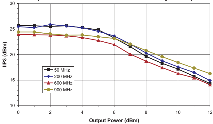
Figure 10: Input IP3 vs. Output Power (T A = +25 °C, V DD = +5 V, 75 Ω system)
