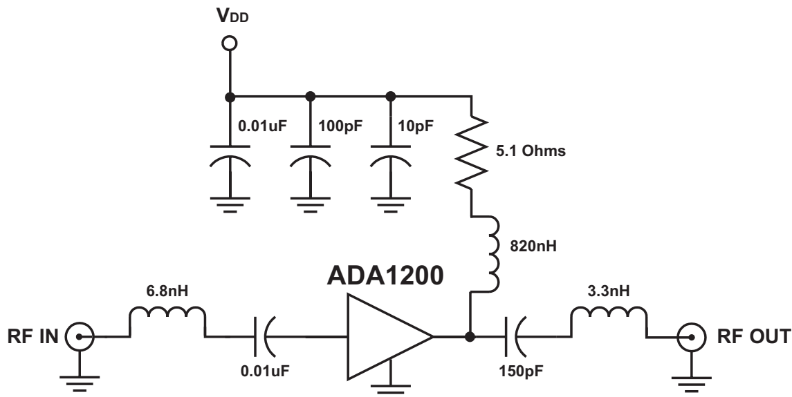
Figure 3: Test Circuit
