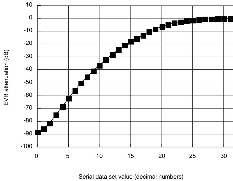
LA74310LP EVR characteristics
