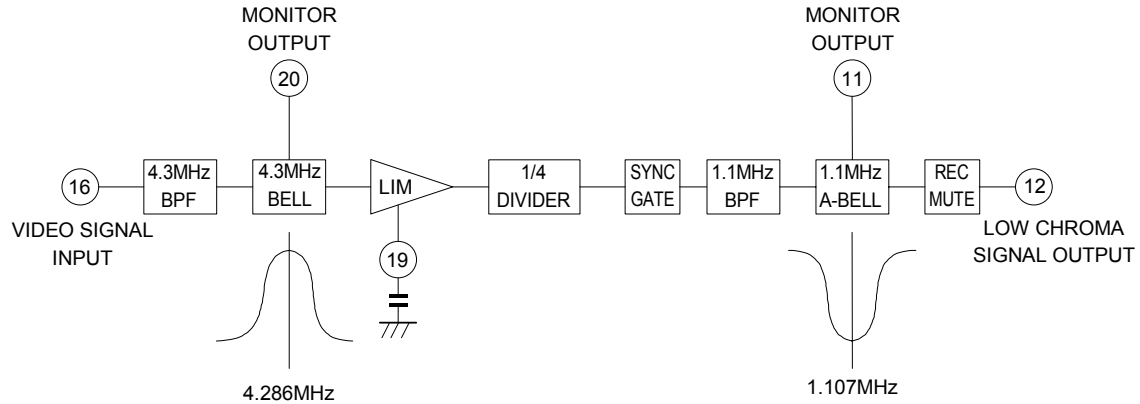
Fig.1 Signal flow in REC mode
