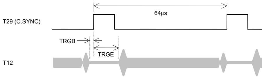
Fig.2 REC mode sync gate timing
