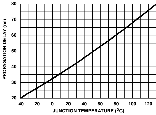
FIGURE 16. UPPER TURN-OFF PROPAGATION DELAY T_{HPLH} vs TEMPERATURE
