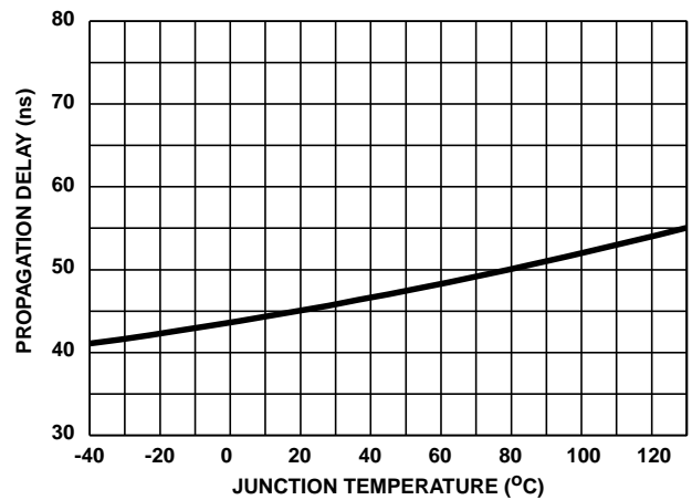
FIGURE 13. LOWER DISABLE TURN-OFF PROPAGATION DELAY T_{DISLOW} vs TEMPERATURE
