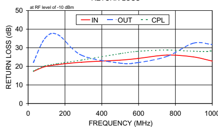
LRDC-10-2-75 RETURN LOSS
