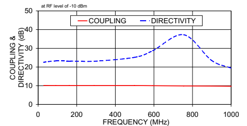
LRDC-10-2-75 COUPLING & DIRECTIVITY
