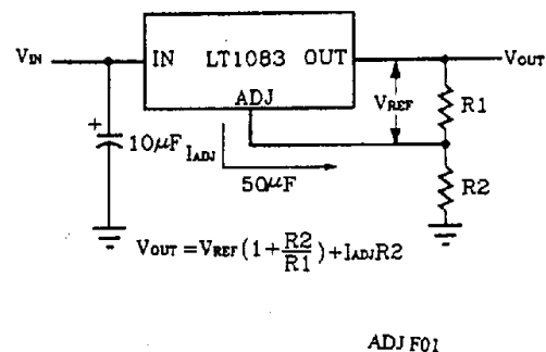
FIGURE 1. BASIC ADJUSTABLE REGULATOR
