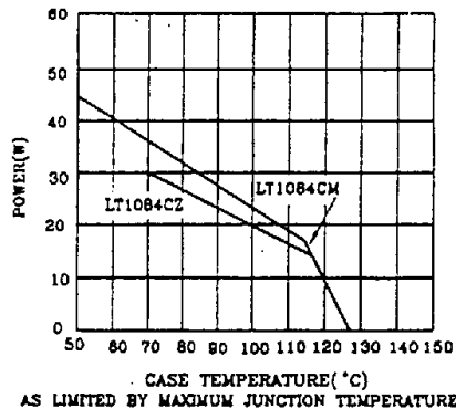
LT1084 Maximum Power Dissipation
