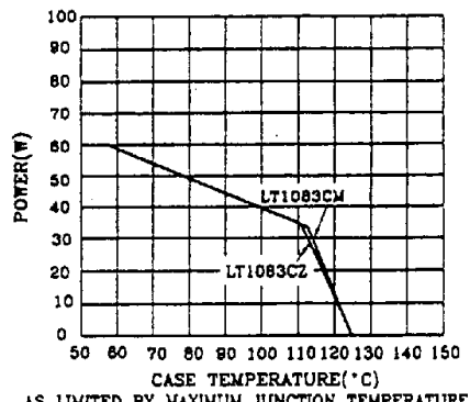
AS LIMITED BY MAXIMUM JUNCTION TEMPERATURE ADJ G15
