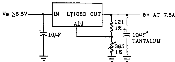
5V, 7.5A Regulator
