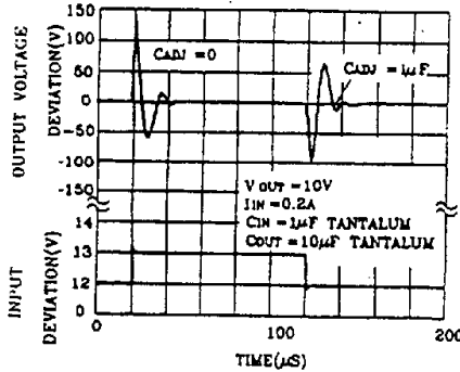
LM1083 Line Transient Response
