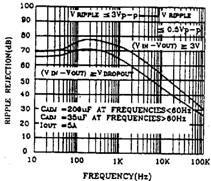
LT1084 Ripple Rejection
