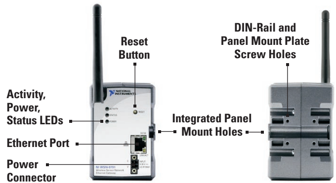
Figure 6. Gateway External Features
