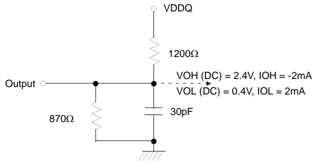
Figure 1. DC Output Load Circuit
