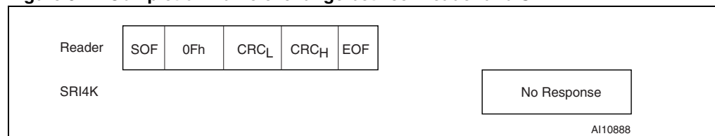
Figure 37. Completion frame exchange between reader and SRI4K
