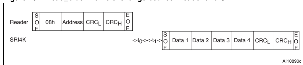
Figure 43. Read_block frame exchange between reader and SRI4K
