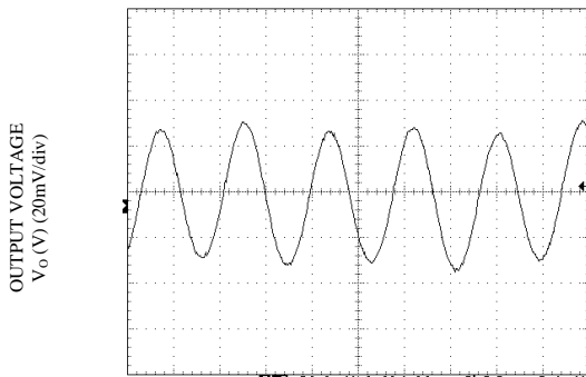
Vo=1.8V, Ta=25°C, Vin=12V, Io = Io,max COUT = 0.1µF // 47 µF ceramic capacitors
