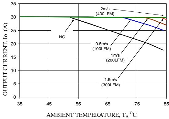
Vo=1.8V, Vin=12V
