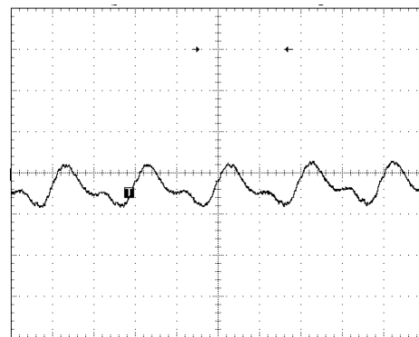
TIME, t (1µs/div) Vo=2.5V, Io = Io,max
