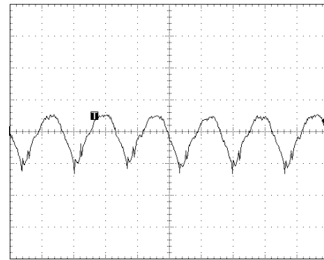
TIME, t (1µs/div) Vo=1.2V, Io = Io,max
