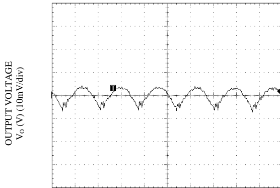
TIME, t (1µs/div) Vo=0.6V, Io = Io,max
