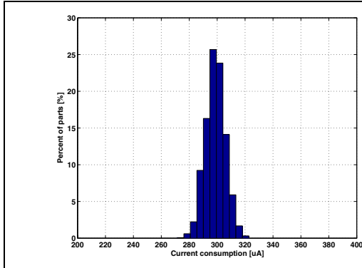
Figure 24. Current consumption in normal mode at 2.5V
