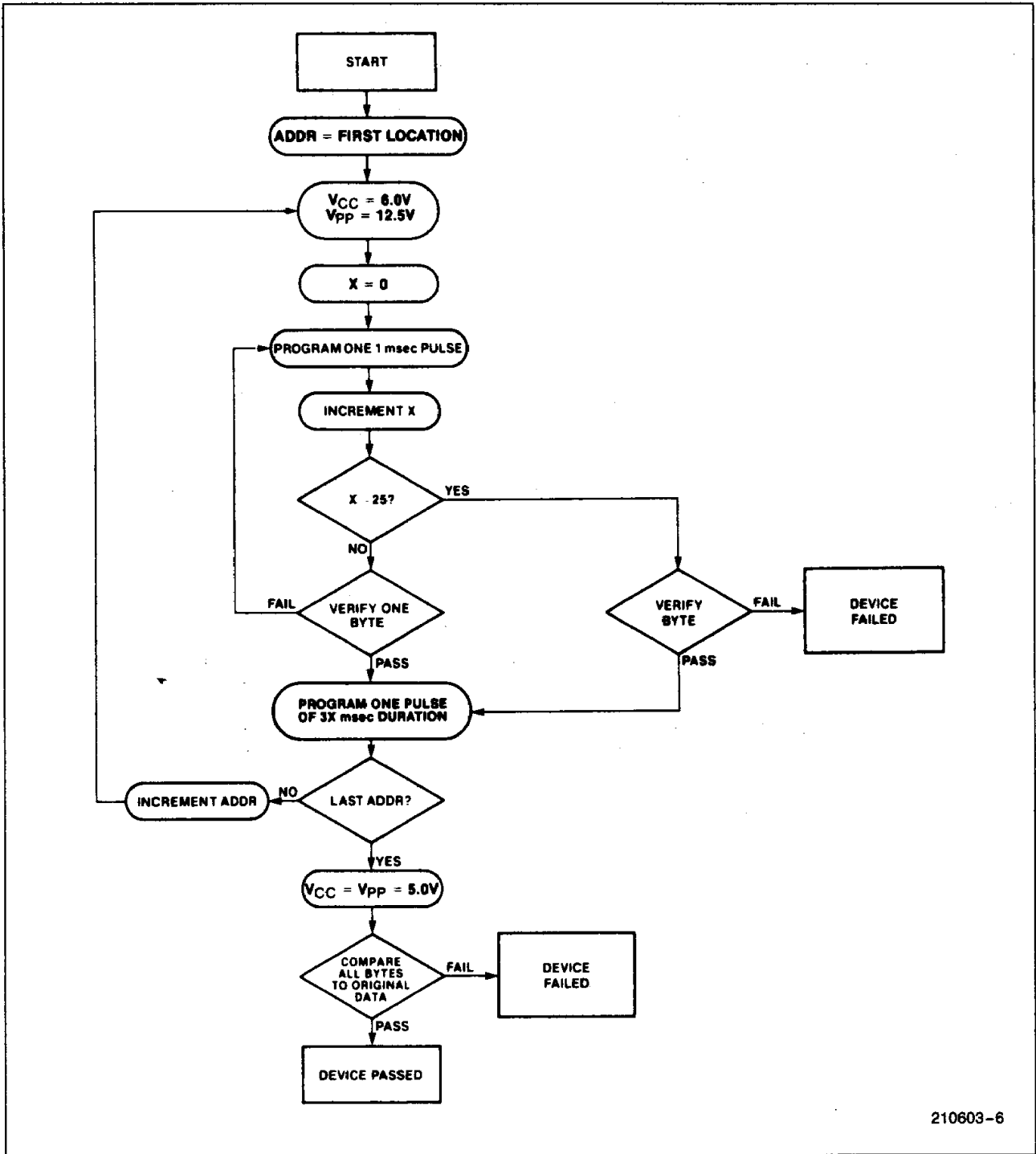
Figure 3. M27128A Intelligent Programming™ Flowchart
