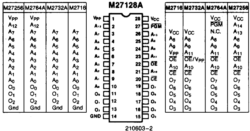
Figure 2. Pin Configurations
